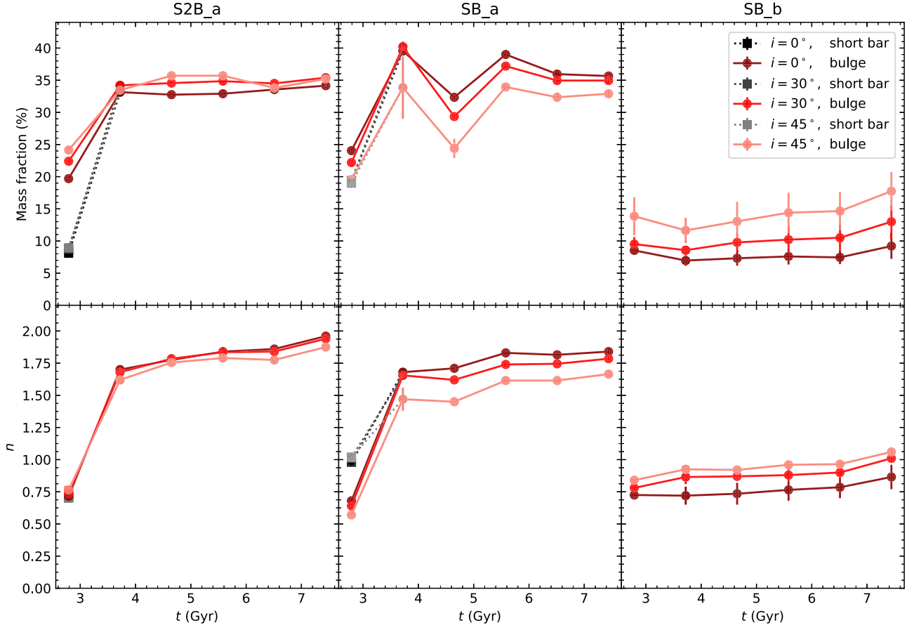
Figure 4. Evolution of the mass fraction (top) and Sérsic index n (bottom) of the bulges in S2B_a, SB_a, and SB_b (from left to right). The results of the short bars are overlaid for models S2B_a and SB_a. The error bars represent the results obtained using Ferrers and Sérsic bars; the dots mark their average values. The error bars are generally smaller than the size of the symbols, except for the case of i = 45^\circ . The squares show the mass fraction and Sérsic index of the short bars. From dark to light colors, we vary the inclination angle from i = 0^\circ to 45^\circ .
