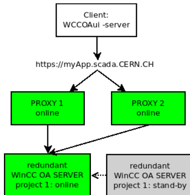
Figure 3. Two proxies and a redundant WinCC OA project.
