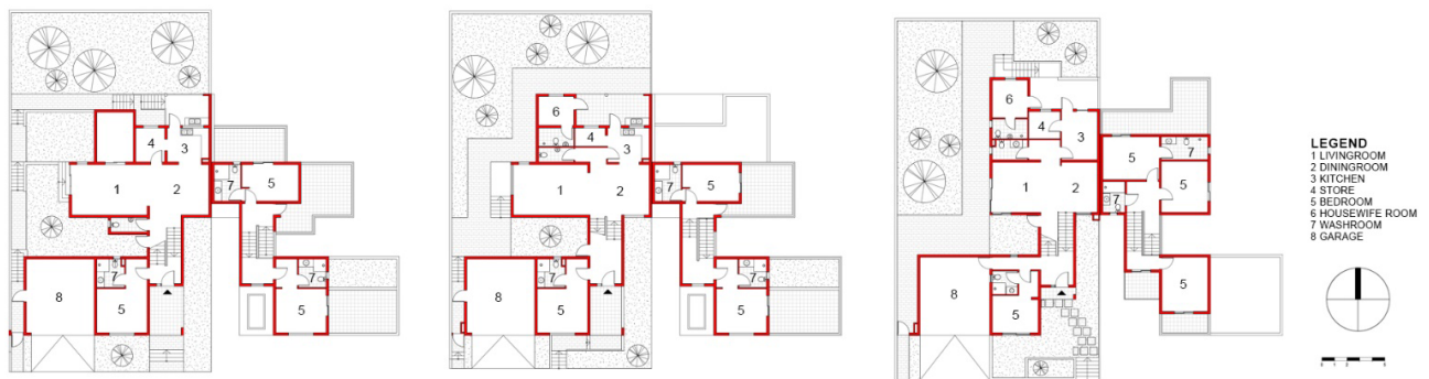
Figure 53. The Umudugudu Kigali Vision: Ground and first floor twin houses (3-4 Bedrooms). Drawing by Manlio Michieletto.
