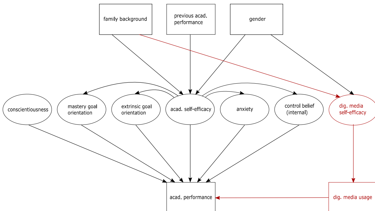
Figure 1: Path diagram of theoretically assumed relationship of constructs.
