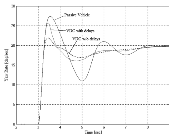
Figure 12: Comparison of vehicle response (yaw rate) during step steer for a passive vehicle, a vehicle including an ideal VDC without delays in the actuation system, and a vehicle actuated by a commercial VDC unit (HIL test)
