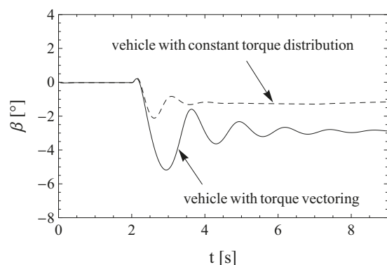
Figure 9: Step steer response ( 0^\circ - 100^\circ ) evaluated at \alpha_x=3 \text{ m/s}^2 and V=90 \text{ km/h} . The dashed curve refers to a vehicle with a constant torque distribution whereas the black curve refers to a torque vectoring strategy that consists in the torque distribution proportional to the vertical load acting on the wheel
