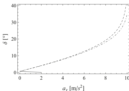
Figure 5: The steering-wheel angle \delta [°] as a function of the lateral acceleration a_y [m/s 2 ] for the three torque distribution strategies, evaluated at a value of the longitudinal acceleration a_x = -5 m/s 2 . The solid curve refers to strategy i), the dashed curve refers to strategy ii), and the dot-dashed curve refers to strategy iii).
