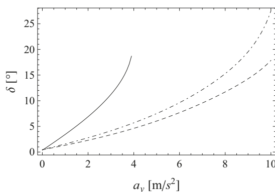
Figure 4: The steering-wheel angle \delta [°] as a function of the lateral acceleration a_y [m/s 2 ] for the three torque distribution strategies, evaluated at a value of the longitudinal acceleration a_x = 5 m/s 2 . The solid curve refers to strategy i), the dashed curve refers to strategy ii), and the dot-dashed curve refers to strategy iii).
