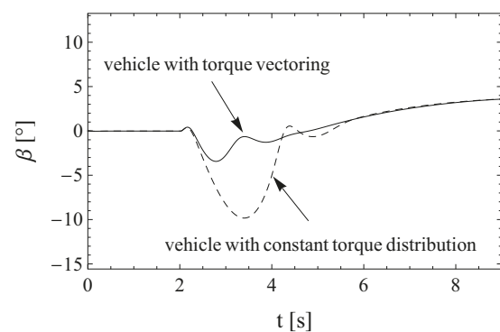
Figure 10: Step steer response ( 0^\circ - 100^\circ ) evaluated at \alpha_x=-3 \text{ m/s}^2 and V=90 \text{ km/h} . The dashed curve refers to a vehicle with a constant torque distribution whereas the black curve refers to a torque vectoring strategy that consists in the torque distribution proportional to the vertical load acting on the wheel
