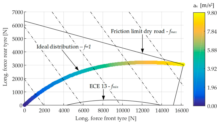
Figure 7. The figure shows the ideal braking force distribution, whereby the colorbar refers to the specific deceleration levels. The figure also reports the limit set by the R13 ECE (Economic Commission for Europe) [25] and the friction utilisation limit on dry road. Iso-deceleration conditions are represented by dash-dotted lines.
