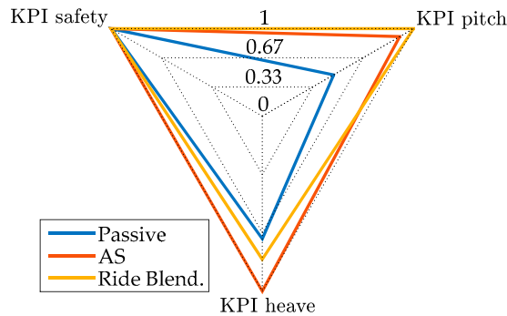
Figure 10. Key performance indexes improvement for the straight line braking maneuverer.
