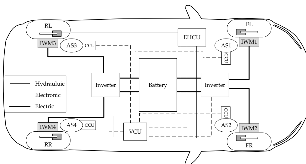
Figure 2. Configuration of the full electric vehicle under analysis. IWM—In-wheel motor; AS—Active suspension; CCU—Corner control unit; EHCUC—Electrohydraulic control unit; VCU—Vehicle control unit.
