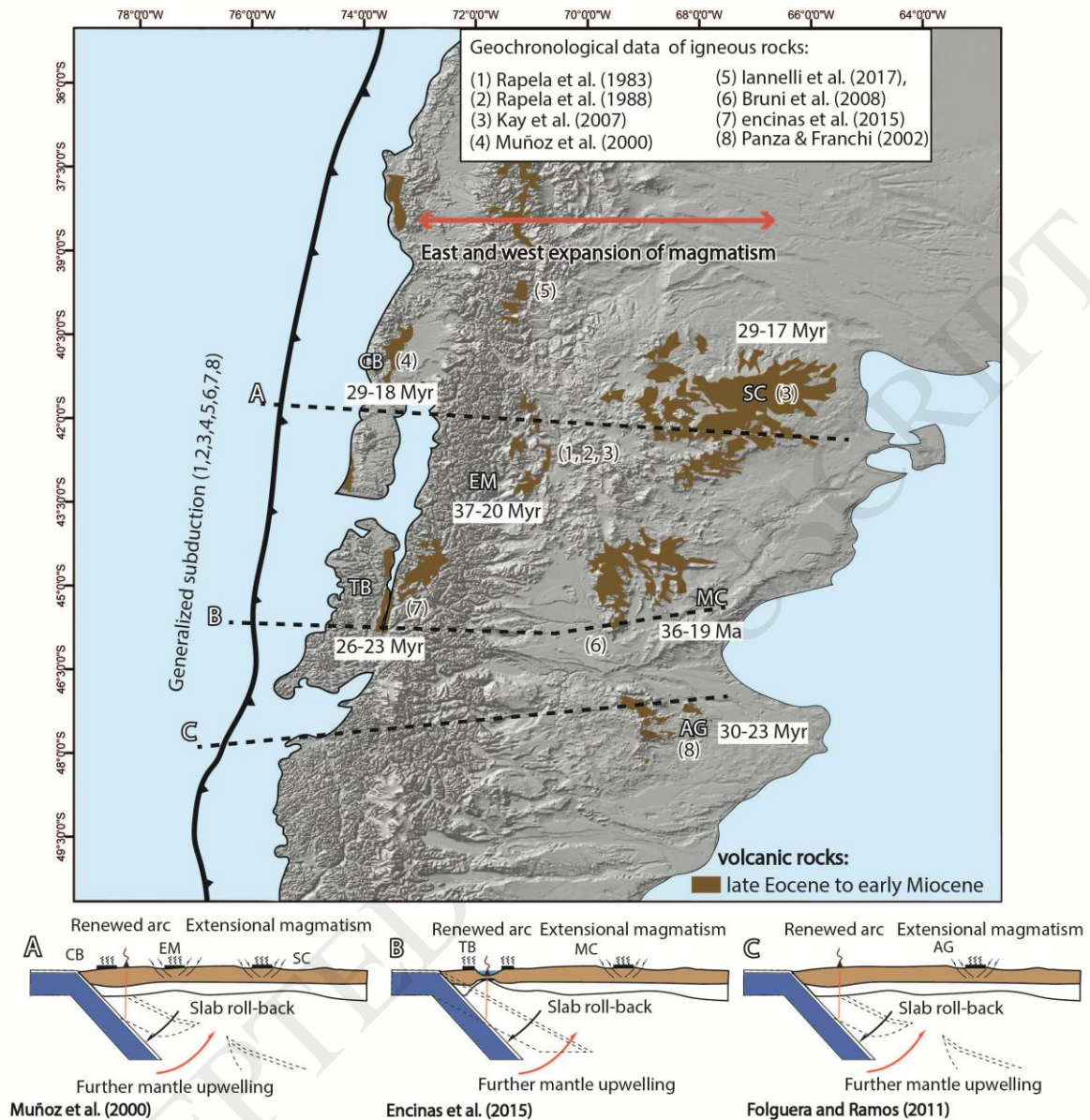
Figure 3. Tectonic setting of Patagonia during ~36 to 18 Myr from 39°30'S to 48°S. At this time synextensional magmatism spread in an east and west direction from the intraplate area to the forearc zone. A to C are three schematic cross sections summarizing the proposed geodynamic contexts between ~36 to 18 Myr. Profiles A, B, and C are the general models for the latest Eocene to early Miocene time interval, where tectonomagmatic activity has been linked to mantle upwelling induced by slab-roll back during rapid and
