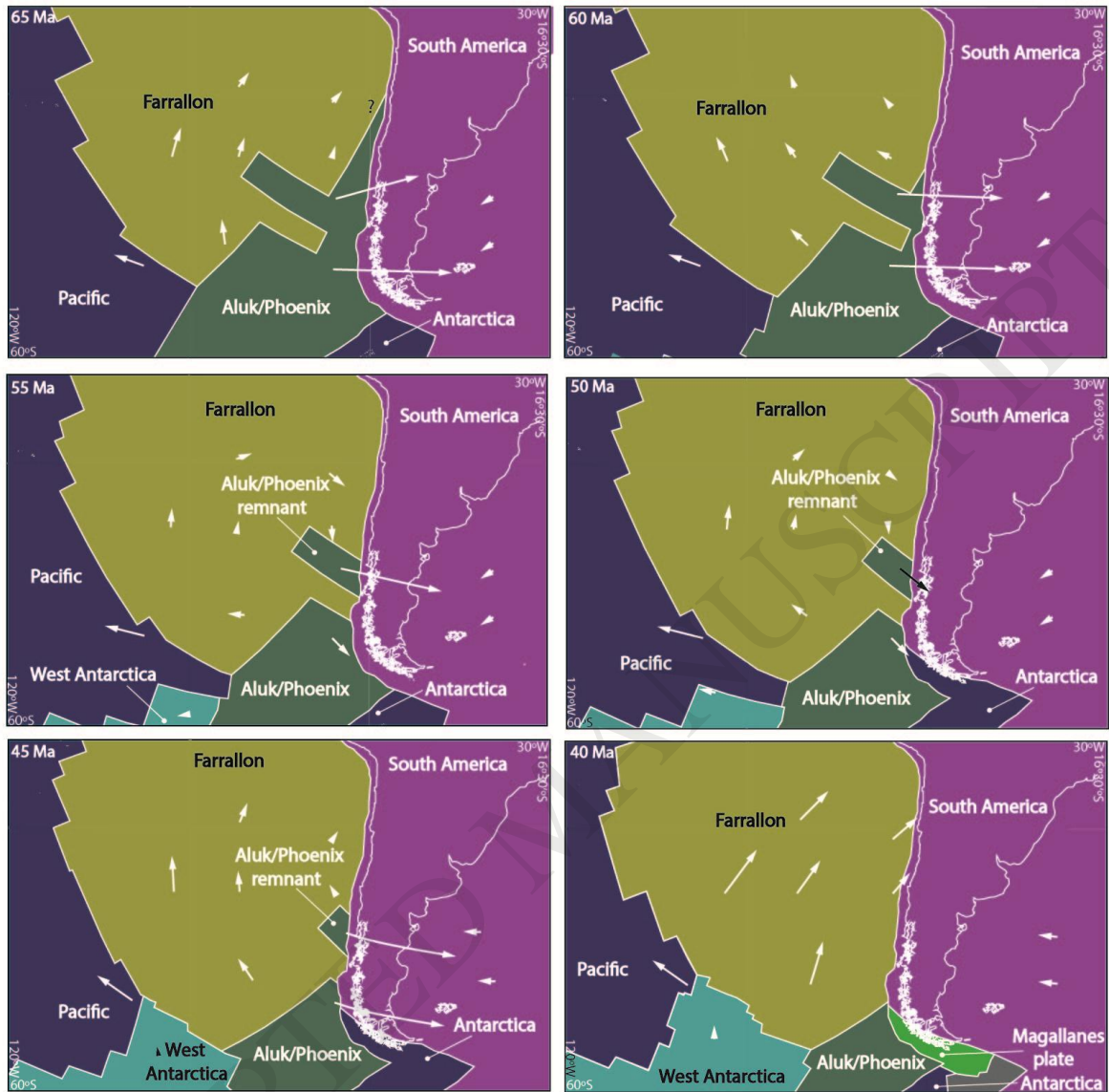
Fig. 6. Proposed reconstruction of the interaction of the Farallon/Aluk(Phoenix) mid-ocean ridge and the South American margin in Paleogene times shown in Mercator projection. The reconstruction was obtained by modifying previous model of Müller et al. (2016) by including the existence of a transient Aluk(Phoenix) plate remnant. The early Paleogene geological record of two potential slab windows at 39°S-44°S and 46°30'-48°S, and plate-wide contraction linked to normal subduction between those segments were used as
