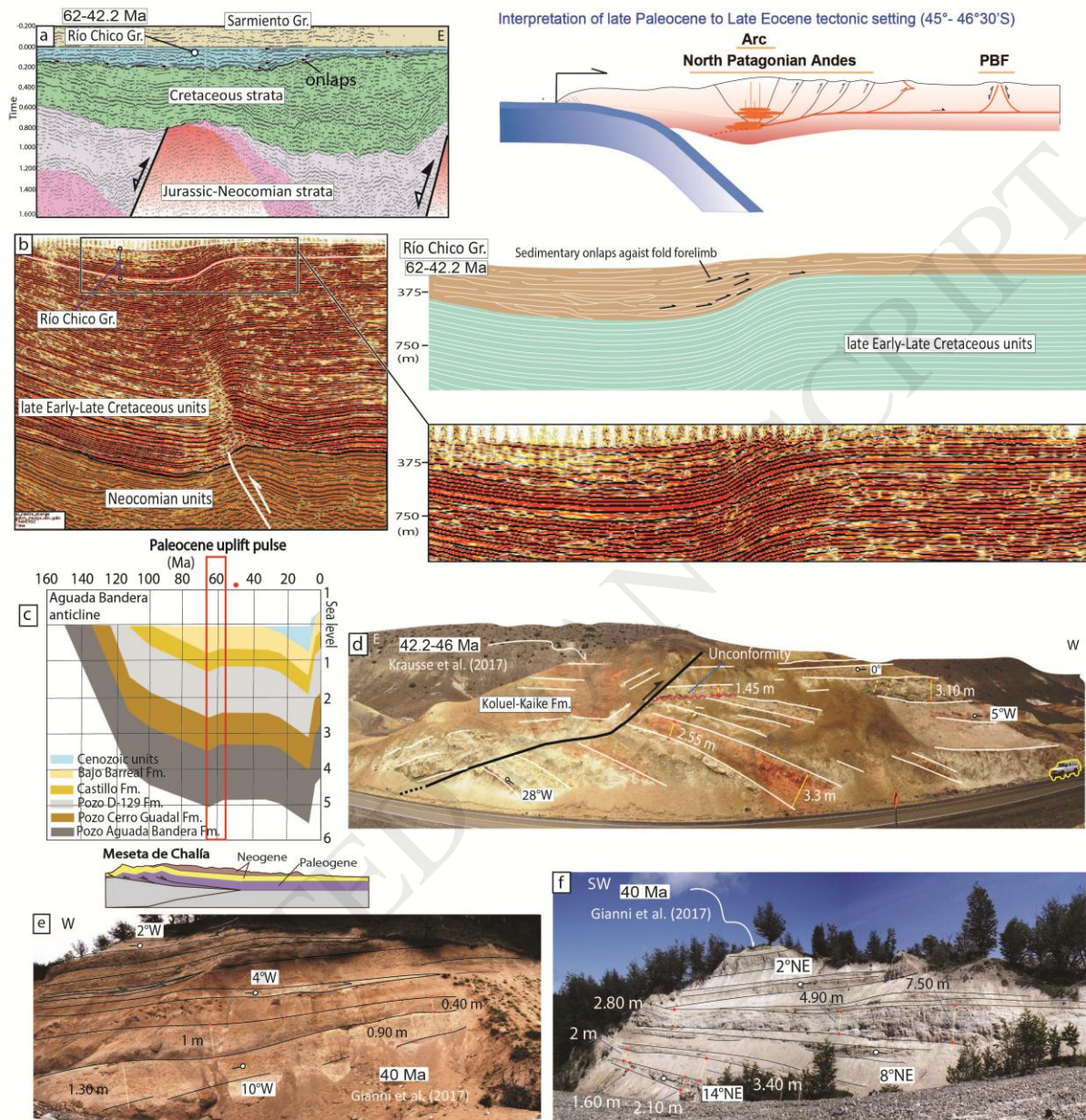
Figure 5. Structural evidence of late Paleocene-Eocene contraction between 45°S to 46°30'S. a) and b) are examples of late Paleocene-Eocene growth of contractional structures observed in seismic lines. a) is modified from Gianni et al. (2015a) and b) is from this work. c) Subsidence curve of the Aguada Bandera anticline depicting an uplift stage during Paleocene times. Modified from Cevallos et al. (2016). d) Eocene syncontractional
