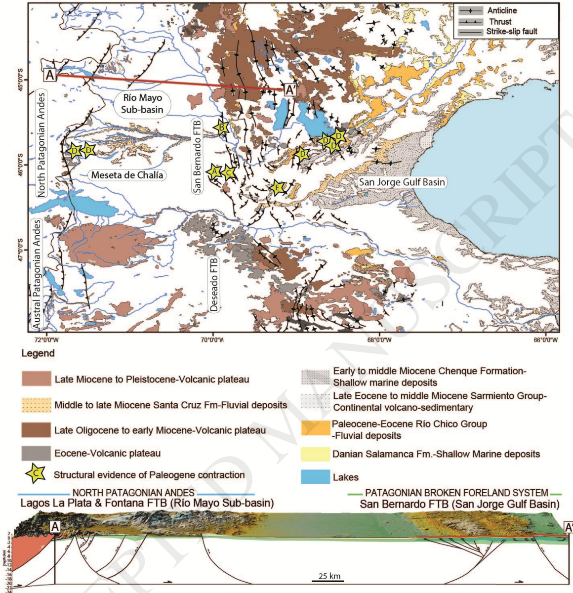
Figure 4. Geological sketch map showing the main morphostructural units and Cenozoic formations from Patagonia between \sim 44^\circ to 48^\circ S. Modified from Gianni et al. (2017). Yellow stars are locations where structural evidences of Paleogene contraction have been documented in field and/or seismic reflexion surveys. References in the stars are: A: Paredes et al. (2006), B: Navarrete et al. (2015), C: Cevallos et al. (2016), D: Gianni et al. (2017), E: This study.
