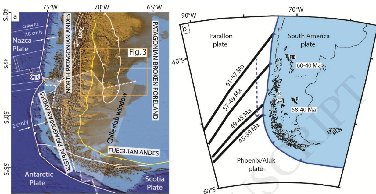
Figure 1. a) Tectonic setting of the Patagonia showing the North and Austral Patagonian Andes, and the broken foreland area. Abbreviations are CTJ: Chile triple junction, LOFZ: Liqueñe-Ofqui fault zone, DM: Deseado Massif and NPM: North Patagonian Massif, FTB: Fold-thrust belt. b) Southward sweeping of the Farallon–Phoenix/Aluk mid-ocean ridge during Paleogene times according to the recent reconstruction of Eagle and Scott (2014) and as previously suggested by Cande and Leslie (1986). Slab window related magmatism is represented in black polygons. Abbreviations are: PIB: Pilcaniyeu magmatic belt, P: Posadas basalt, MCC: Meseta de Chile Chico basalts, B: Balmaceda basalts. See figure 2 for references to geochronological data.
