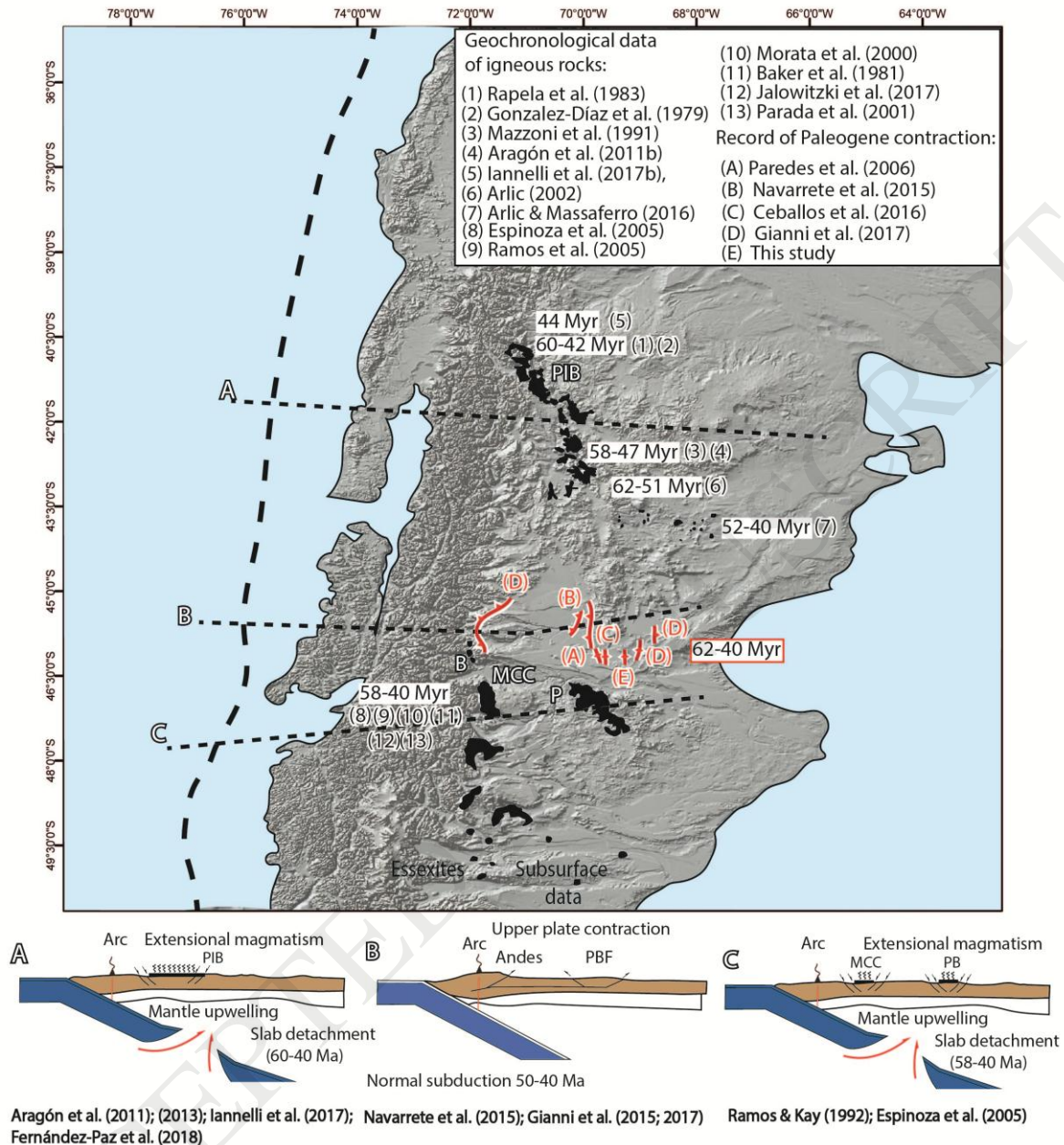
Figure 2. Tectonic setting of Patagonia during the ~60 to 40 Myr time interval from 39°30'S to 50°S. Synextensional within-plate igneous rocks were mostly emplaced in two segments, one at 39°S to 44°S and the other from 46°30'S to 50°S. In between the latter segments, contraction from the plate margin to the intraplate area took place at those times and within-plate magmatic activity was practically absent. A to C are three schematic cross
