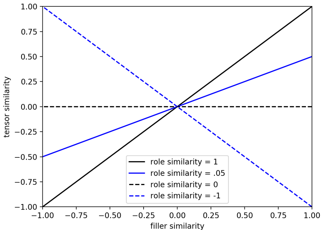
Figure S1. Cosine similarity of two role-filler pairs bound by tensor-product as a function of role and filler similarity.
