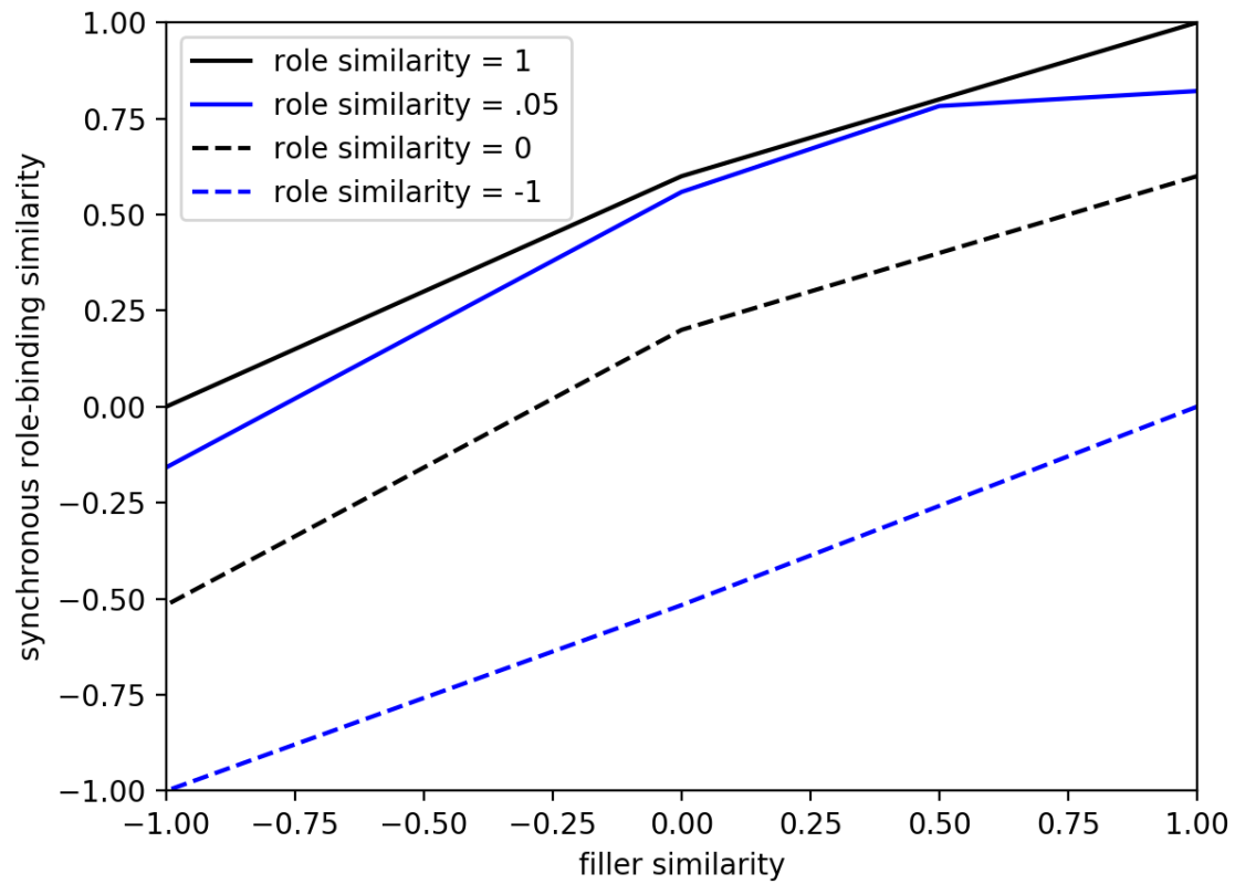
Figure S2. Cosine similarity of two role-filler pairs bound by synchrony as a function of role and filler similarity.
