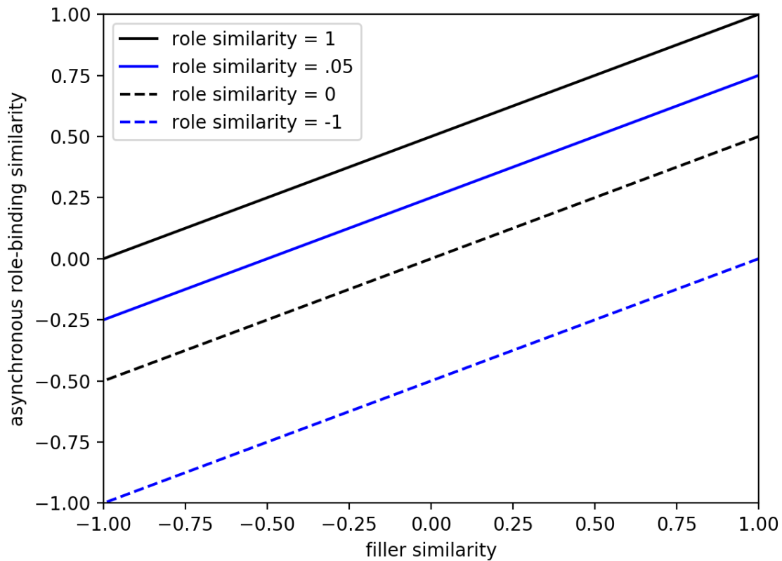
Figure S3. Cosine similarity of two role-filler pairs bound by asynchrony as a function of role and filler similarity.
