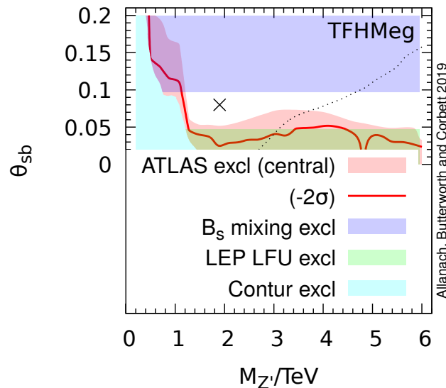
Fig. 6.3 Constraints on the TFHMeg, including the constraint from direct Z' \rightarrow \mu\mu searches at ATLAS, in the \theta_{sb} vs. M_{Z'} plane. Here, the value of the coupling g_F is fixed to the central value from the fit to the NCBA's. Constraints from other electroweak precision observables such as the \rho -parameter are not included in this plot.
