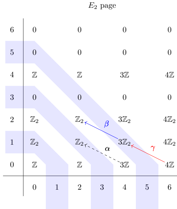
Fig. 7.2 The E_2 page of the Atiyah-Hirzebruch spectral sequence for G = G_{SM} . We see that there is only a single entry relevant to the computation of \Omega_5^{Spin}(BG_{SM}) , with a map ( \gamma ) going in and a map ( \beta ) going out.
