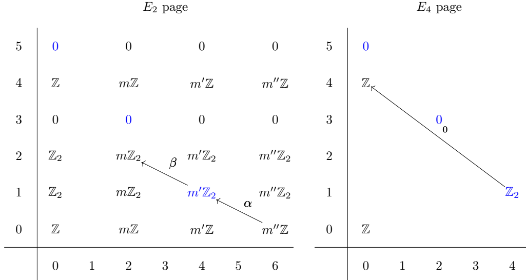
Fig. 7.5 The E_2 and E_4 pages of the Atiyah-Hirzebruch spectral sequence for G = G_{Z'} = U(1)^m \times SU(2) \times SU(3) with all elements and differentials relevant to the calculation of \Omega_5^{\text{Spin}} highlighted.
