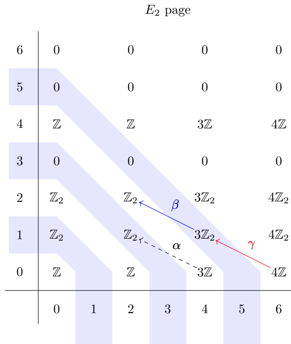
Fig. 7.3 The E_2 page of the Atiyah-Hirzebruch spectral sequence for G = U(2) \times SU(3) , with differentials relevant to the computation of the fourth and fifth spin-bordism groups labelled.
