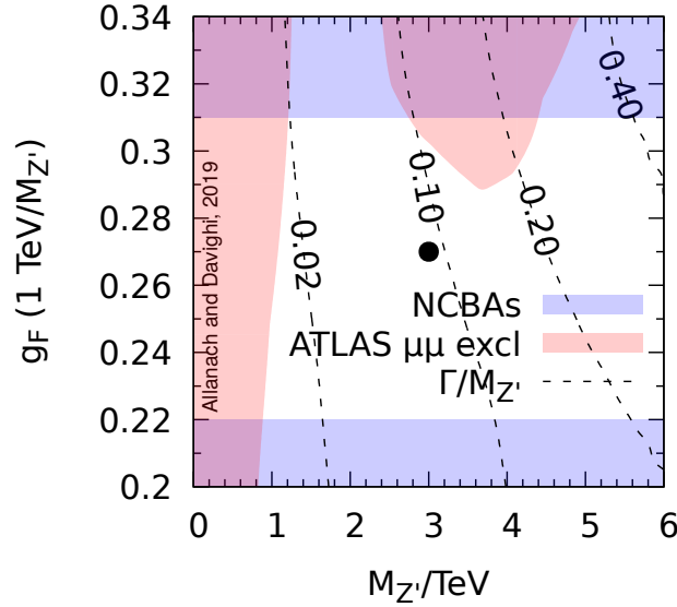
Fig. 6.4 Constraints on parameter space of the DTFHMeg. The white region is allowed at 95% CL. We show the regions excluded at the 95% CL by the fit to NCBAAs, and by the most recent direct searches for Z' \rightarrow \mu^+ \mu^- (labelled by ‘ATLAS \mu\mu excl’). Other constraints, such as from B_s mixing, or lepton flavour universality of the Z boson couplings, are less restrictive than those shown. The example point displayed in Table 6.5 is shown by the dot. Values of \Gamma/M_{Z'} label the dashed line contours, where \Gamma is the width of the Z' . In this plot we have not included bounds coming from electroweak precision observables such as the \rho -parameter, which we plan to compute accurately in future work.
