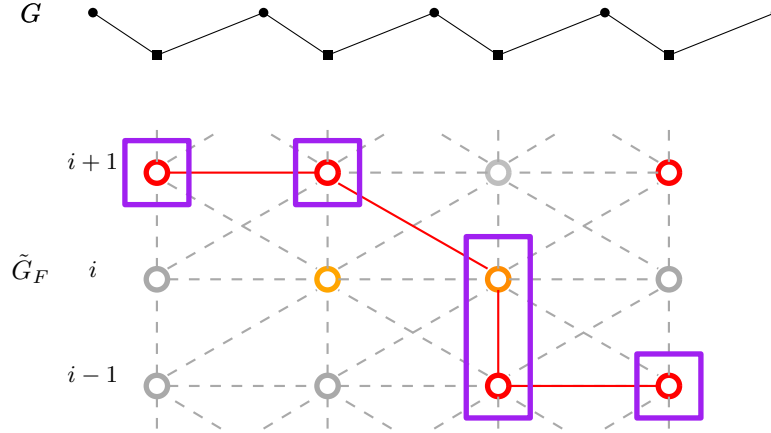
(B) An open path in the site percolation on \tilde{G}_F
