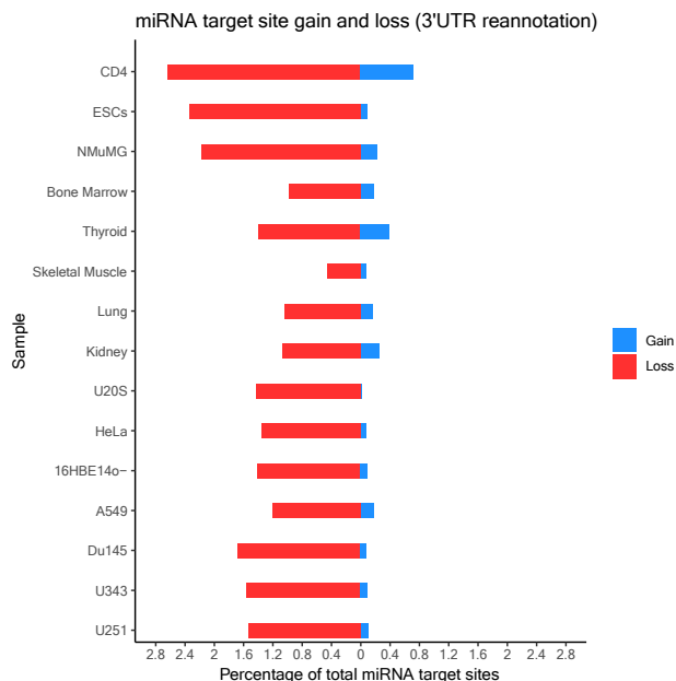
Fig. 4. Total miRNA target site gain and loss when applying FilTar to multiple sample types. FilTar is applied to the protein-coding transcriptome for all annotated human miRNAs for multiple tissues, organs and cell lines. Gained (blue) and lost (red) miRNA target sites is expressed as a percentage of the total number of target sites identified when deriving miRNA from Ensembl 3'UTR annotations.
