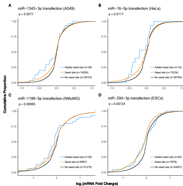
Fig. 2. 3'UTR elongation by FilTar leads to the identification of additional valid miRNA targets. Curves show the cumulative log 2 fold change distributions of i) protein-coding non-target transcripts (black). ii) protein-coding seed target transcripts (orange) and iii) predicted target transcripts deriving from FilTar 3'UTR annotations but not Ensembl 3'UTR annotations (blue). Approximate P-values were computed using one-sided, two-sample, Kolmogorov-Smirnov tests between pre-existing target and newly identified target fold change distributions. Otherwise as in figure 1.
