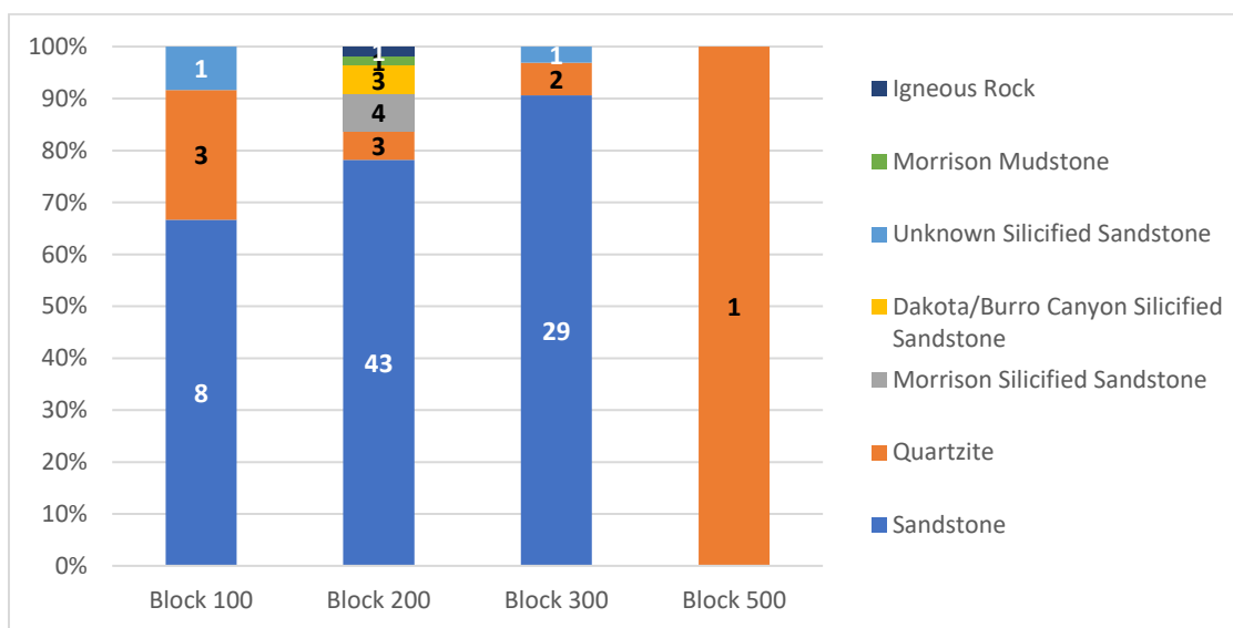
Figure 3.43. Material Type by Architectural Block at The Dillard Site.
