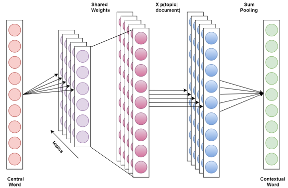
Figure 1: We feed our model a central word as input and predict the context word from it. First we learn separate word embeddings corresponding to each topic, E_{w_t, z_i} . Each of these embeddings are then multiplied with global word embeddings, v_g(w) , weighed in proportion to the topic distribution of the document from which the words have been chosen, and summed up to predict the neighboring context word.
