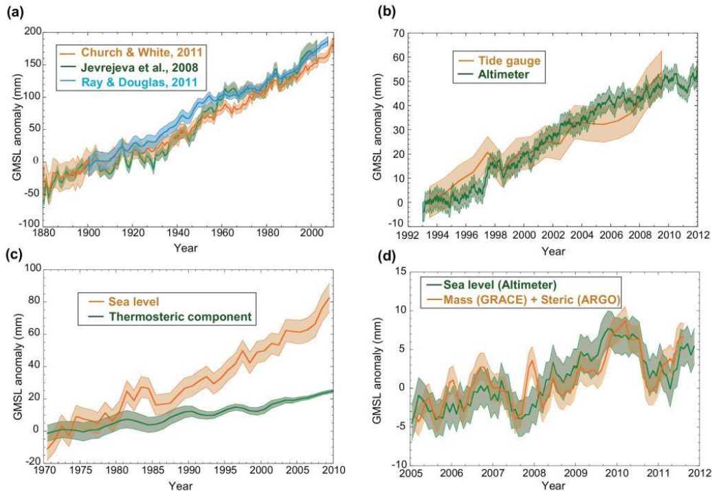
Figure 13: Global mean sea level rise anomalies.
