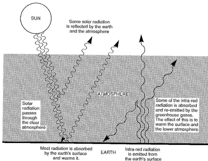
Figure 1: Illustration of Green House Effect
