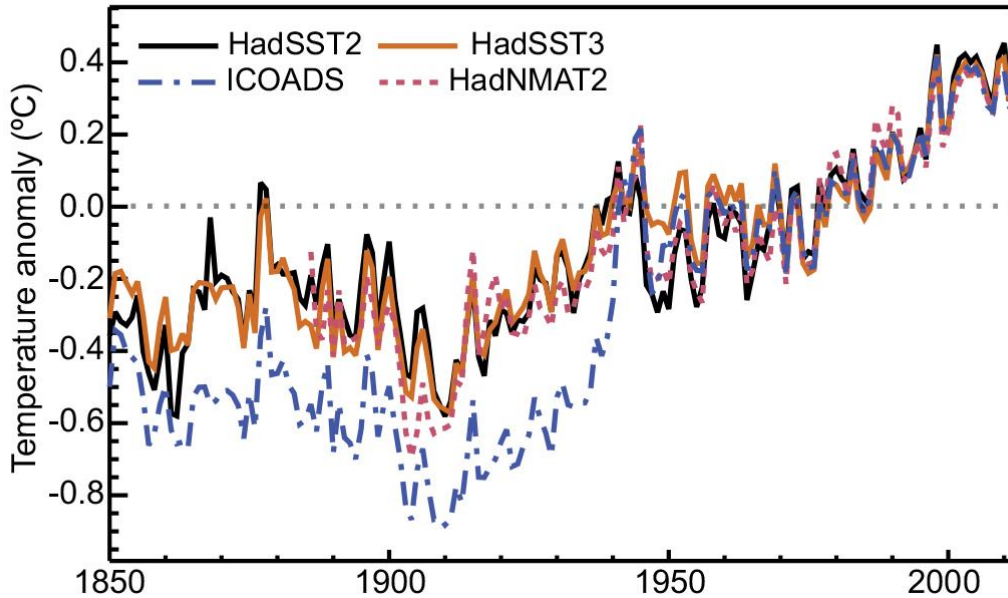
Figure 10: Global annual sea surface temperature anomalies from 1859 to 2005
