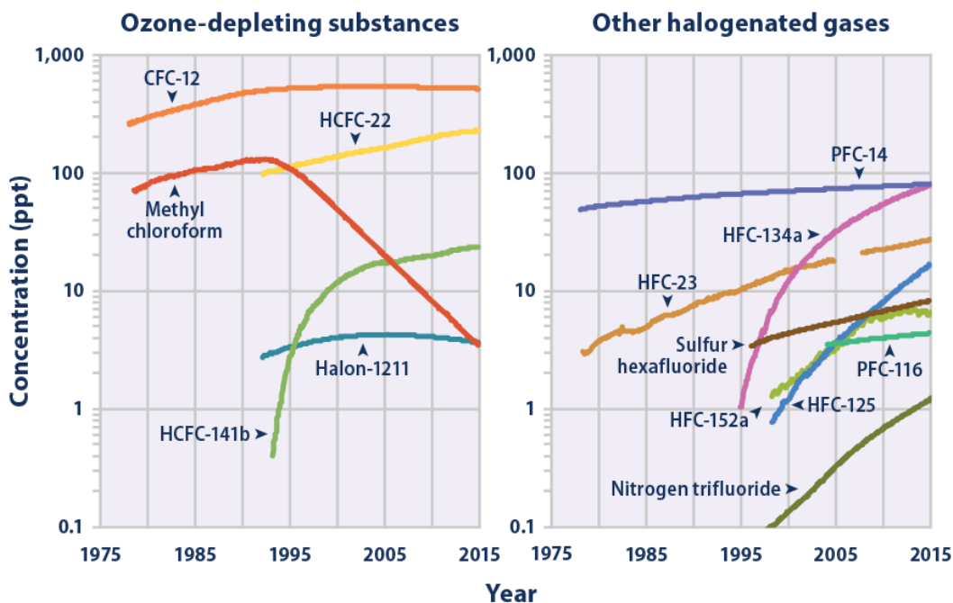
Figure 5: Halo Carbon concentration since 1975
