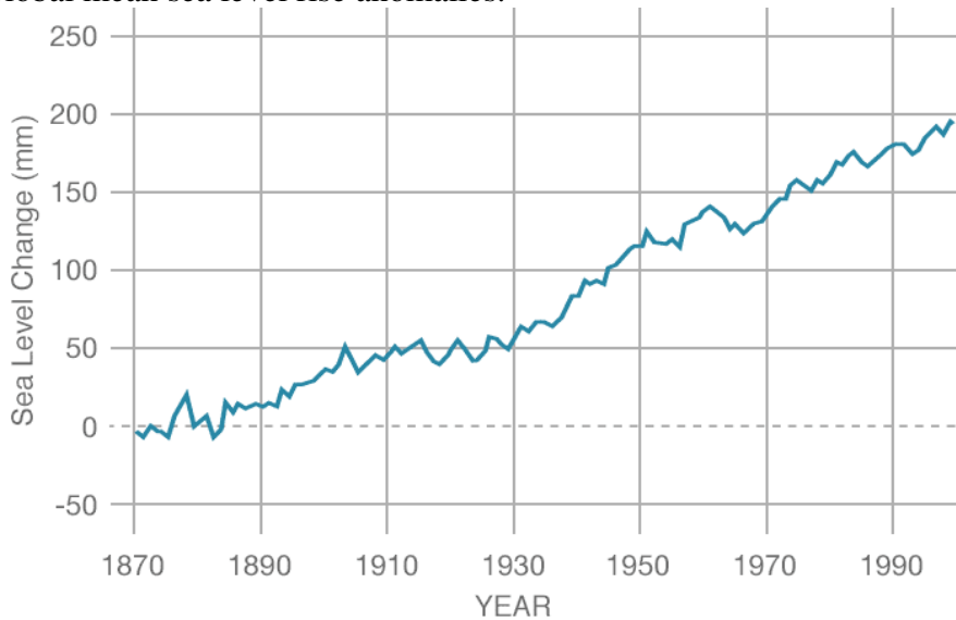
Figure 13: Global mean sea level rise anomalies.
