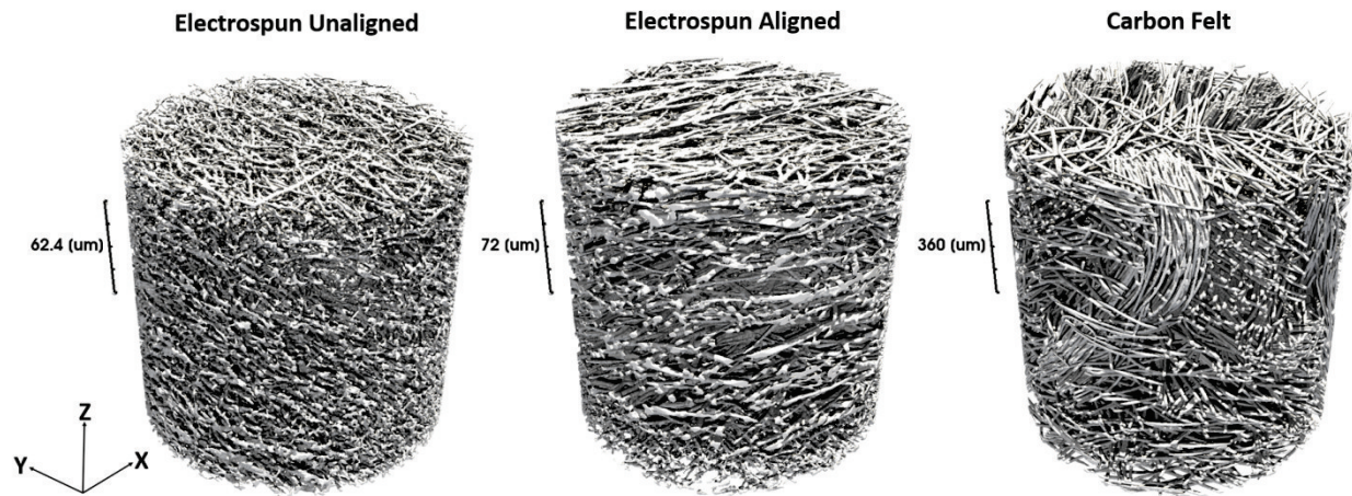
Figure 1: Reconstructed 3D image from X-ray computed tomography. The left image shows the electrospun unaligned material, the middle image shows the electrospun material with anisotropic fibers, the commercially available carbon felt is shown on the right. Note the substantially larger scale bar of the carbon felt image compared to the electrospun materials.
