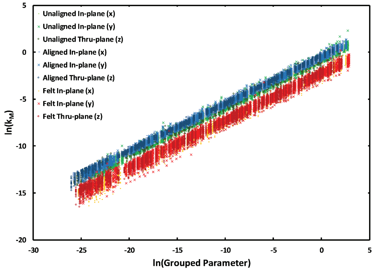
Figure 8: Natural logarithm of the mass transfer coefficient versus natural logarithm of the grouped parameter for all materials in all directions.
