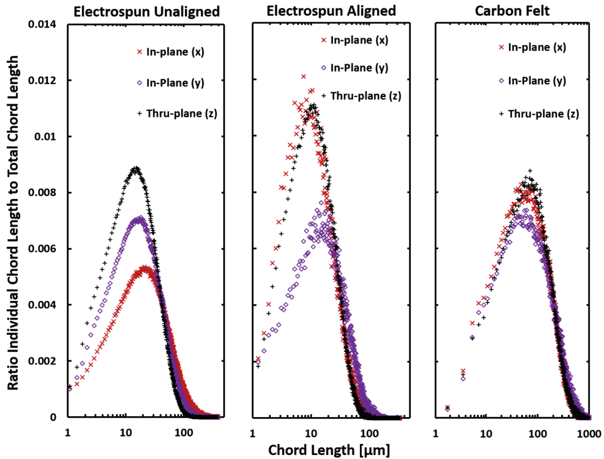
Figure 5: Chord-length distribution in the pore-space for the three materials.
