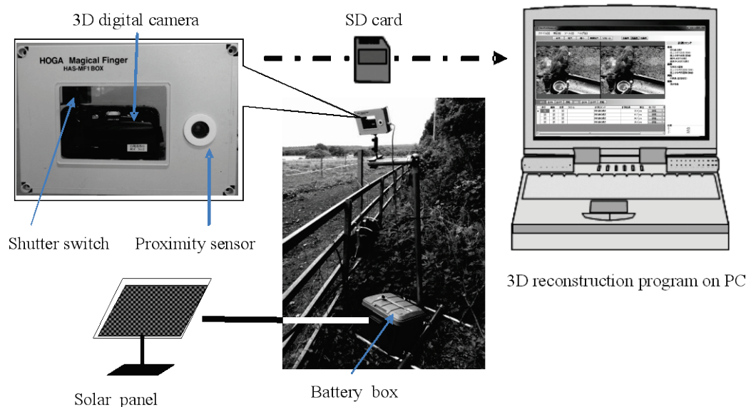
Figure 1. The trail 3D digital camera unit installed near the pasture water sources.
