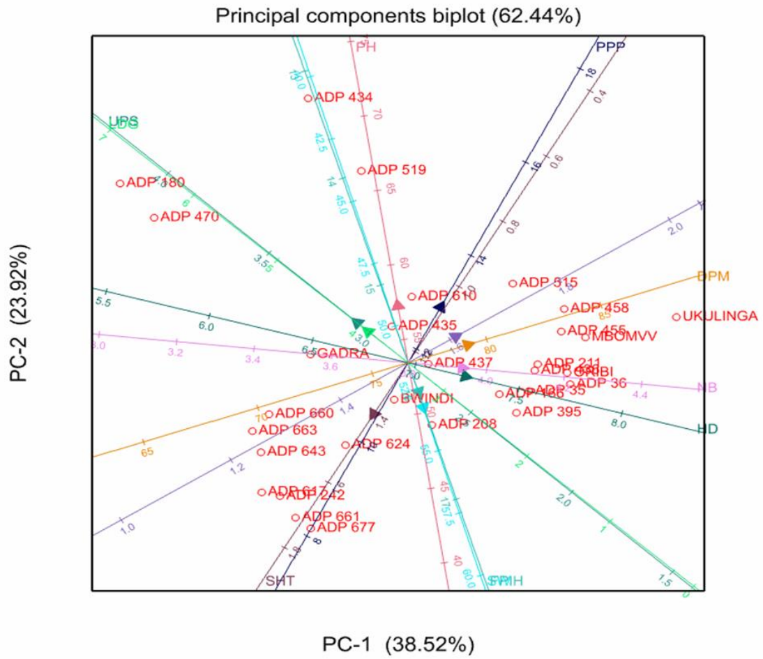
Figure 3.1 Principal components biplot showing genotypic grouping
