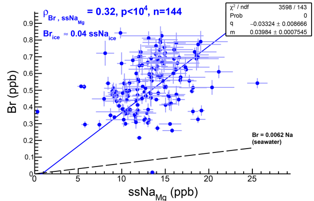
Figure C1. Correlation between bromine and \text{ssNa}_{\text{Mg}} concentrations in the glacial section of the RECAP ice core. The weak positive correlation suggests a common source for the two elements. The slope of the (qualitative, p(\chi^2) \sim 0 ) linear fit indicates significant ( \sim 6 ) enrichment compared to seawater mass ratios (black line).
