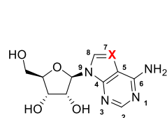
X = N; adenosine, 1 X = CH; tubercidin, 2 purine numbering
