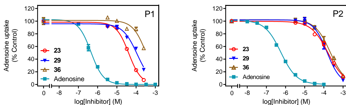
Figure 2: Transporter binding experiments of selected nucleoside analogues with P1 and P2 of bloodstream form T. brucei . The transport of 50 nM [ 3 H]-adenosine by bloodstream forms of T. b. brucei strain B48 (panel P1) or B48 expressing TbAT1/P2 (panel P2) was measured in the absence or presence of increasing concentration of nucleoside analogues. The panels each show a single experiment, performed in triplicate, that is representative of three identical but independent experiments. Error bars are SEM and when not shown fall within the symbol.
