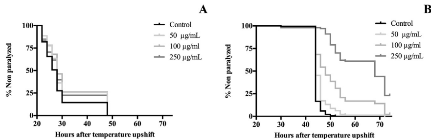
Fig. 4 – Effect of (A) V. cornuta and (B) V. x wittrockiana extracts on A \beta -induced paralysis in transgenic C. elegans CL4176. Three replicates were examined per treatment. Statistical significance difference between the curves was analysed by log-rank (Kaplan–Meier) statistical test which compares the survival distributions between the control and treatment groups. Differences in survival curves between treatment and control groups were found in:(A) 50 **, 100*** and 250* \mu\text{g}/\text{mL} ; (B): 50, 100 and 250 (***) \mu\text{g}/\text{mL} . Differences compared to control group were considered significant at p \leq 0.05 (*), p \leq 0.01 (**) and p \leq 0.001 (***).
