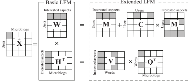
Figure 1: Our extensible Latent Factor Model (LFM)
