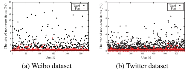
Figure 3: Decomposition alleviated sparsity of user data
