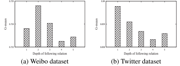
Figure 4: Influence of the depth of followers considered
