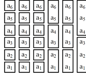
Fig. 5: Illustration of an arbitrary combination of task bins Comb = \{3 \times b_1, 2 \times b_2, 1 \times b_3\} .
