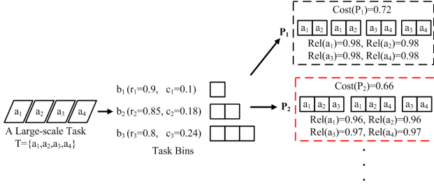
Fig. 4: Illustration of the SLADE Problem
