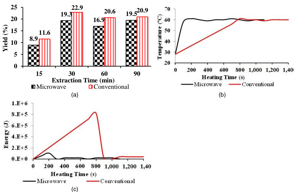
Figure 2: Comparison study for microwave and conventional heating techniques (a) yield vs. extraction time, (b) temperature vs. heating time for 15 min extraction, and (c) energy vs. heating time for 15 min extraction. The maximum estimated standard deviations of the measured data: Yield \pm 2 %, Temperature \pm 1 °C.
