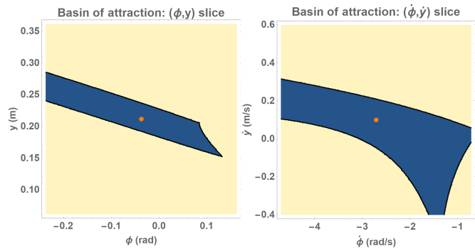
Fig. 6. Two slices of the numerically-computed basin of attraction when the hybrid mode sequence is enforced, using parameters given in Table III (left - in the (\varphi, y) plane, right - in the (\dot{\varphi}, \dot{y}) plane). The blue region indicates the basin, and the center orange dot corresponds with the fixed point \bar{\mathbf{x}}^I of the map H^I . The enforcement of the hybrid mode sequence is a very conservative assumption for real-world implementation, as the ability to move through transient hybrid mode sequences is an inherent affordance of legs that provides robustness and motivates their use on machines.
