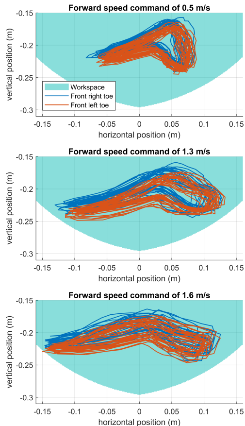
Fig. 11. Toe kinematic trajectories for the front legs in the local hip frame show that at running speeds of 1.6 m/s, the leg linkage is going close to singularity. This represents a constraint on maximum running speed, as the leg runs out of workspace to sweep the leg backwards in stance. Faster running with the control strategy of Section II could be achieved by either using longer legs to increase the workspace or by achieving shorter stance durations through increasing the applied vertical stance force. In future work we will investigate the addition of a spine morphology to provide this added workspace without detracting from the hip’s torque generation affordance.
