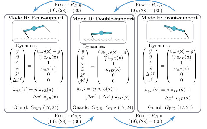
Fig. 3. The hybrid dynamical system (3) representing the model shown in Figure 2 with state \mathbf{x}_i = (\mathbf{x}^I T, \mathbf{x}_i^H T)^T . The state component \mathbf{x}^I (10) gives the state related to the mass center's vertical height and pitch states, as well as mode timers; while \mathbf{x}_i^H (11) gives the mass center's horizontal position and velocity, as well as the horizontal toe positions. The guards G_{i,j} and resets R_{i,j} are introduced in (17) and (19), respectively, and further specified in (24)-(25) and (29)-(31) to decouple the hybrid transitions as shown in Figure 4. Approximation 1 and the choice of force laws (21), (33) decouple the continuous dynamics as shown in Figure 4. There is no flight phase due to actuator limitations when running at speed on the physical machine as described in Section V-A, however accounting for an aerial mode instead of double support would yield a system for which a similar control strategy as described in Section IV could be applied. Note that the horizontal toe locations indicated by \Delta x^i and x^i , i \in \{f, r\} – unchanged by the continuous dynamics – are set by the resets as control inputs.
