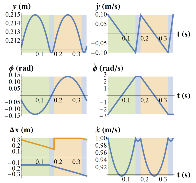
Fig. 5. Traces of the hybrid periodic orbit over a full stride using the parameters of Table III at a commanded speed of 1 m/s. The background color indicates the mode (4). Green is F, blue is D, and yellow is R. In the \Delta x graph, the blue trace gives \Delta x^r while the orange trace gives \Delta x^f (12). Notice that deviations in body height y and forward speed \dot{x} are quite small, indicating a valid Approximation 1 as discussed in Section III-D and a small value of \xi from Table II.
