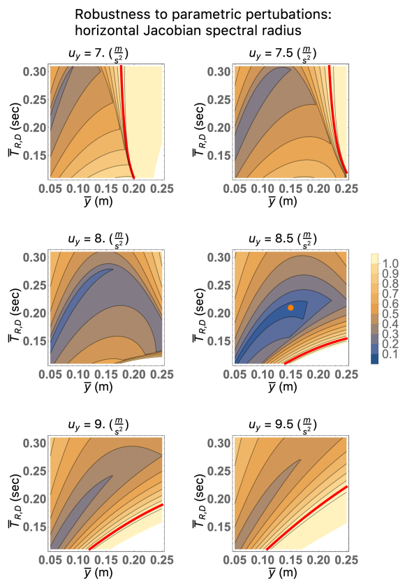
Fig. 8. Slices of the Jacobian spectral radius of H^H evaluated at the appropriate fixed point with parametric perturbations in the parameters \bar{y} , T_{R,D} , and u_y – the only parameters entering into the Jacobian. This analysis uses numerical parameter values given in Table III as the unperturbed values. Here the control is being done using the unperturbed parameters, showing the robustness of the control scheme to parametric uncertainty. The distance from the orange dot in the lower-left plot (representing the unperturbed parameter values) to the red line (indicating slices of the edge of stability) demonstrates that the controller can withstand sizable perturbations in parameter space before going unstable.
