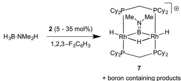
Scheme 4. Attempted dehydrocoupling of H_3B\cdot NMe_2H and formation of [[Rh(\mu-dcpm)]_2(\mu-H)(\mu-BNMe_2)][Al\{OC(CF_3)_3\}_4] ( 7 ). [Al\{OC(CF_3)_3\}_4]^- anion not shown.
