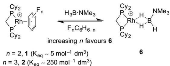
Scheme 3. Formation of [Rh(dcpm)(\eta^2-H_3B\cdot NMe_3)][Al\{OC(CF_3)_3\}_4] ( 6 ) ( n = 2, 3 ). [Al\{OC(CF_3)_3\}_4]^- anion not shown.
