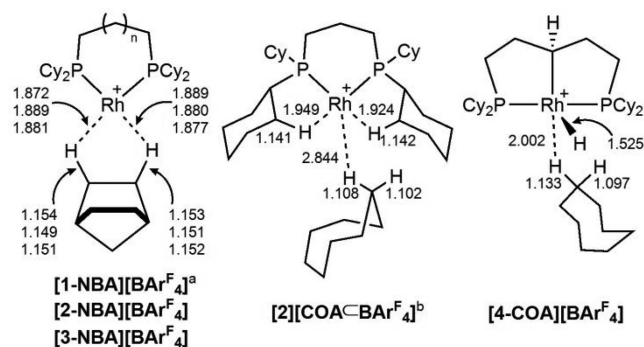
Figure 10. Computed distances (Å) involving key H atoms in [X-NBA][BARF 4 ] a (X = 1, 2, and 3; n = 0, 1, and 2, respectively), [2][COACBARF 4 ], and [4-COD][BARF 4 ]. a data are for endo -C–H bonds: all exo -C–H bond distances fall between 1.094 and 1.100 Å. b a structure based on optimization of the major component.
