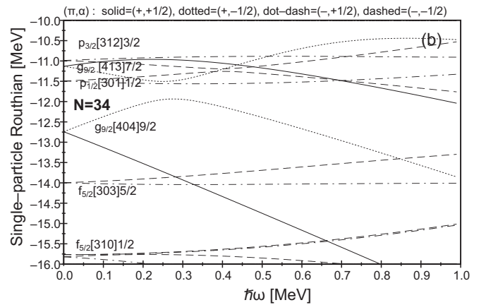
FIG. 21. Woods-Saxon (a) proton and (b) neutron single-particle Routhians calculated versus rotational frequency (for \beta_2 = 0.33 and \gamma = 30^\circ ) for ^{66}\text{Ge} . For the rotational frequency \hbar\omega \approx 0.7 MeV single proton orbitals: g_{9/2}([404]9/2) and f_{5/2}([303]5/2) crosses, this configuration couples to a spin of 7^- .
