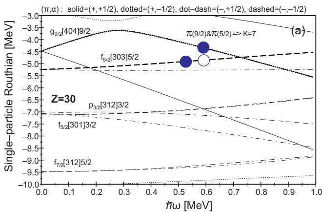
FIG. 21. Woods-Saxon (a) proton and (b) neutron single-particle Routhians calculated versus rotational frequency (for \beta_2 = 0.33 and \gamma = 30^\circ ) for ^{66}\text{Ge} . For the rotational frequency \hbar\omega \approx 0.7 MeV single proton orbitals: g_{9/2}([404]9/2) and f_{5/2}([303]5/2) crosses, this configuration couples to a spin of 7^- .
