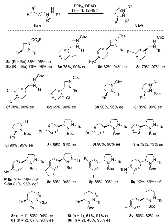
Figure 3. Cyclic hydrazines 8a-v made by Mitsunobu ring closure. a Reaction with DIAD in place of DEAD (for full details, see Supporting Information).
