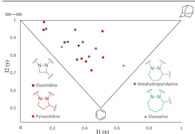
Figure 5. Principal moments of inertia (PMI) plot of hydrazines 10a-q indicating their molecular shapes. Mean PMI indicated (◆).
