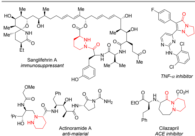
Figure 1. Representative examples of bioactive molecules containing cyclic hydrazine and hydrazide frameworks (highlighted in red).
