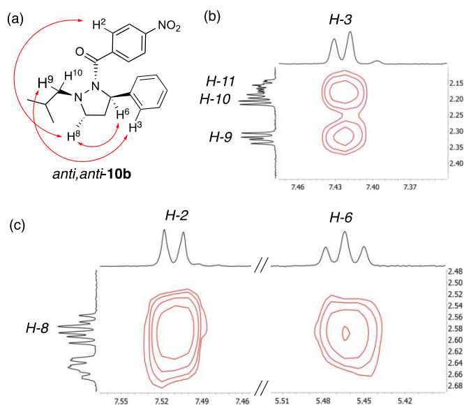
Figure 7. Solution-state structure of 10b derived by 1 H- 1 H NOESY spectroscopy (600 MHz, C 6 D 6 , 343 K): (a) anti,anti -representation of 10b with key NOEs indicated (red arrows). (b) Expansion of the NOESY spectrum highlighting cross-peaks between H-3 and H-9 and possibly H-10. (c) Expansion of the NOESY spectrum highlighting key cross-peaks between H-8 and H-2, and H-8 and H-6.
