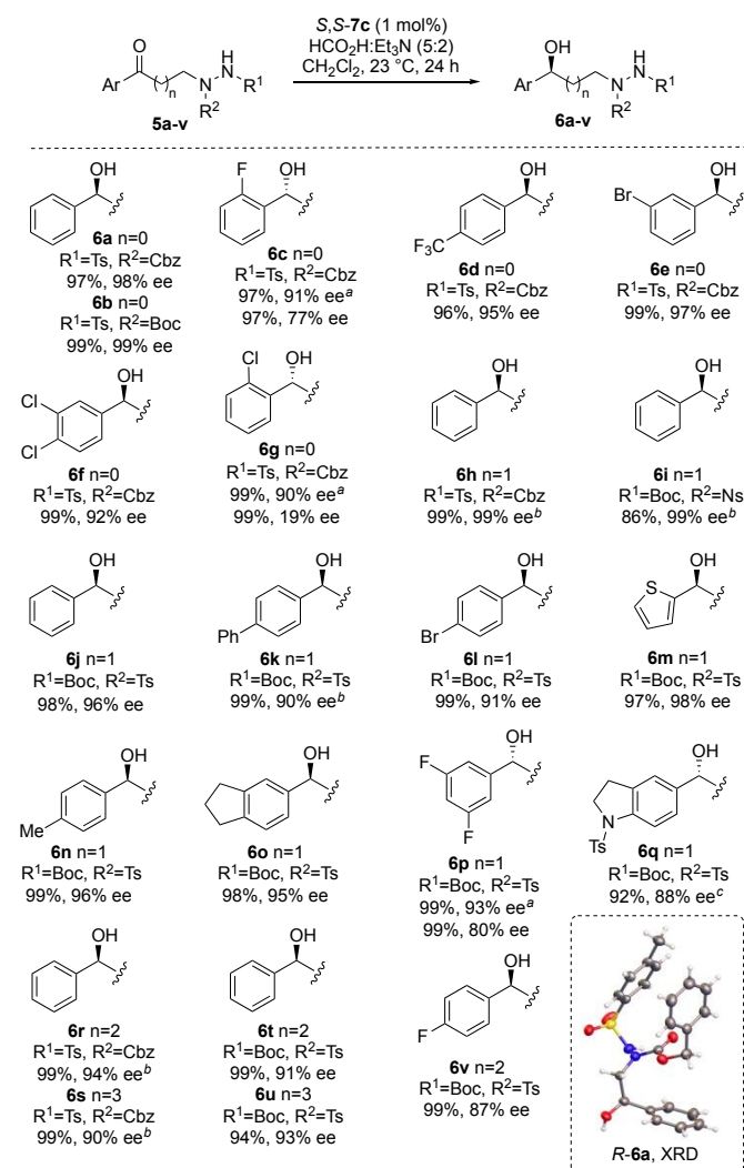
Figure 2. Ru-catalyzed ATH of hydrazone-containing ketones. a Using R,R -7f. b ee determined after cyclization to 8 . c Using R,R -7c.
