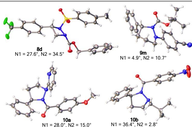
Figure 6. Representative XRD structures of the cyclic hydrazines with measured values for the pyramidalization of the two ring nitrogens (N1 and N2). 18
