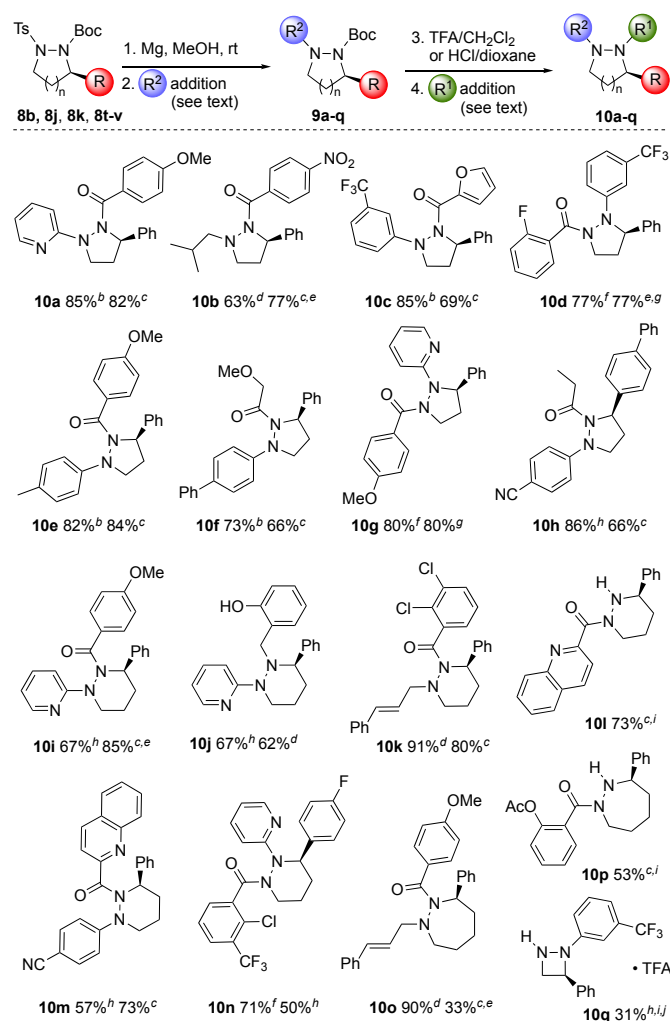
Figure 4. N-Functionalization of enantioenriched cyclic hydrazines and hydrazides. a Isolated yields for two-step syntheses of 9 and 10 respectively. b ArBr, XPhosPd(crotyl)Cl (5 mol%), NaOtBu, toluene, 90 °C, 20 h. c RCOCl, DIPEA, CH 2 Cl 2 , 0 °C to rt, 18 h. d RCHO, NaBH(OAc) 3 , THF, rt, 20 h. e Enantiomeric excess determined by chiral HPLC. f RCOCl, CH 2 Cl 2 , rt, 18 h. g ArBr, BippyPhosPd(allyl)OTf (5 mol%), Cs 2 CO 3 , toluene, 90 °C, 20 h. h ArBr, Pd(OAc) 2 (5-10 mol%), Xantphos (10-20 mol%), NaOtBu, toluene, 90 °C, 20 h. i Yield over 3 steps after Boc removal. j The Boc and Ts groups are transposed in the starting material 8b .
