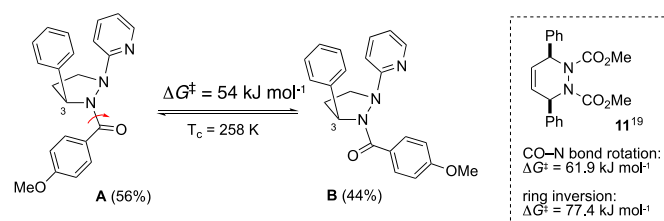
Scheme 2. Likely origin of fluxional behaviour seen in 10a .
