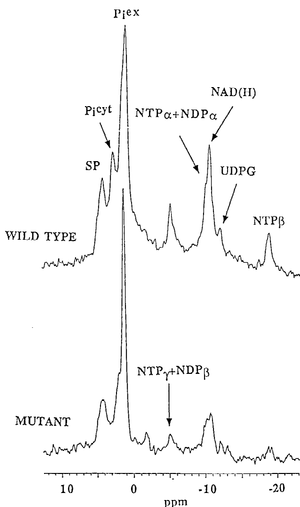
Figure 2. ^{31}\text{P} NMR spectra acquired during anaerobic glycolysis of E. coli strains PPA305 (top spectrum) and PPA316 (bottom spectrum). Spectra were obtained using 40^\circ pulse and a relaxation delay of 0.2 s, other parameters as described in Materials and Methods. Abbreviations: SP: sugar phosphate; \text{P}_i^{\text{cyt}} : intracellular inorganic phosphate; \text{P}_i^{\text{ex}} : extracellular inorganic phosphate; NTP: nucleoside triphosphate; NDP: nucleoside diphosphate; NAD(H): nicotinamide adenine dinucleotide; UDPG: uridine-diphosphoglucose.
