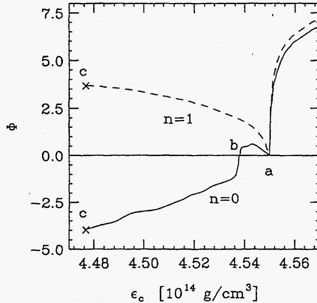
FIG. 2. Pulsation frequencies for n = 0, 1 measured by \Phi(x) \equiv \text{sign}(x) \log(1 + |x|) where x \equiv (\omega_n / \text{sec}^{-1})^2 as a function of central star density in the vicinity of strange dwarfs having inner crust density equal to neutron drip. For \Phi < 0 , the squared frequency is negative and the mode unstable.
