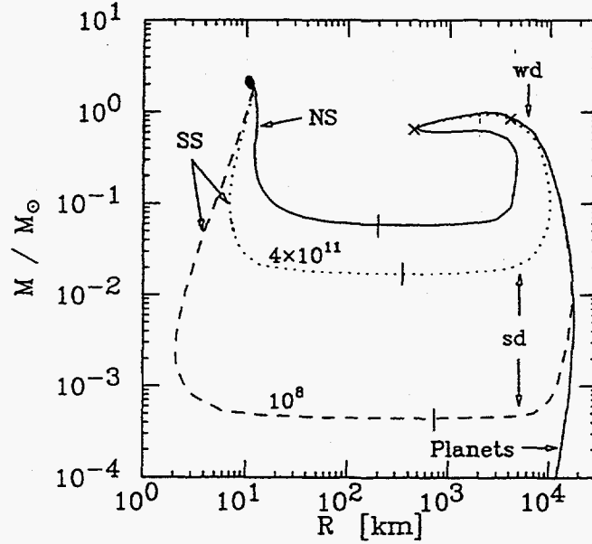
FIG. 1. Neutron star (NS) - white dwarf (wd) sequence, (solid line). Two strange star (SS) - strange dwarf (sd) sequences, for which the inner crust density of nuclear material has the indicated values (in \text{gm}/\text{cm}^3 ). The higher value is the drip density. Vertical bars mark minimum mass stars. Crosses mark termination of the strange star sequences where the strange core shrinks to zero. At those points they become identical to ordinary white dwarfs.
