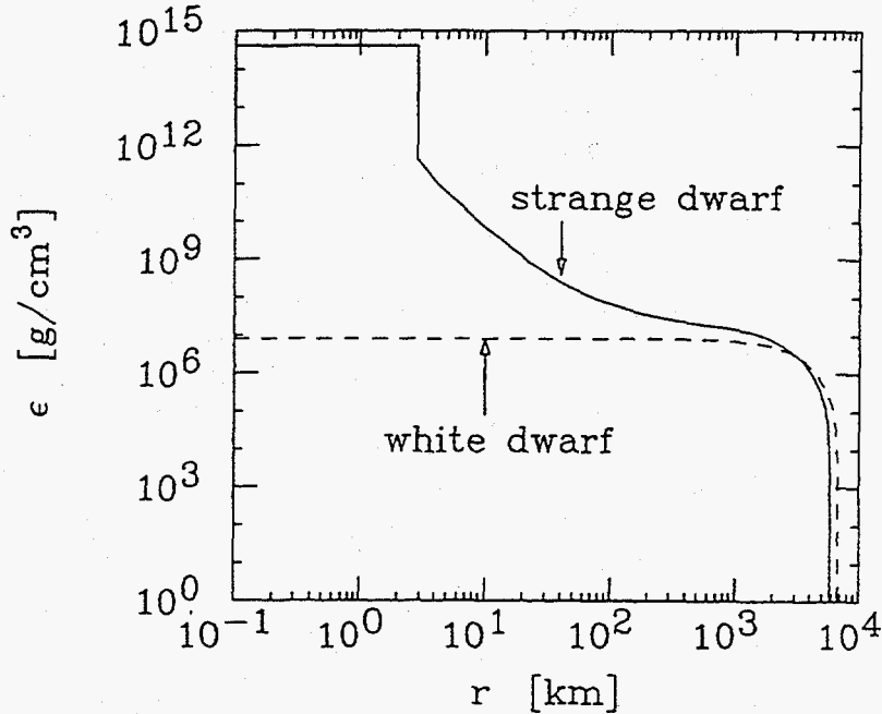
FIG. 3. Mass-energy profile of a strange dwarf and a white dwarf of the same mass, 0.6M_{\odot} . Quark core of strange dwarf is the structure within 3 kilometers. Outside is nuclear material of inner density equal to the neutron drip density.
