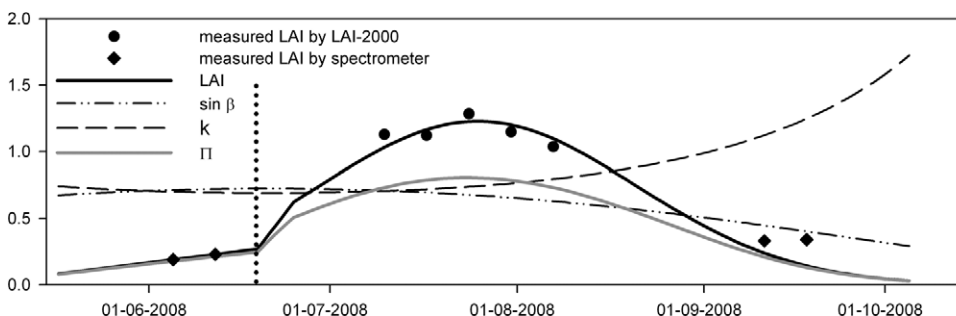
FIGURE 4. Development of measured and interpolated LAI, the sinus of the sun elevation ( \beta ), the extinction coefficient ( k ) and the canopy period ( \Pi ) during the modeling period. The dotted line indicates the start of the bud break.
