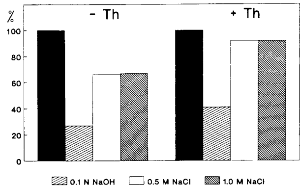
Figure 3. Envelope–pSSU interaction is salt resistant. Outer envelope membranes were incubated with radiolabelled pSSU. After re-isolation, the membranes were treated with different concentrations of NaCl or NaOH either before thermolysin (–Th) or after thermolysin (+Th) treatment. The amount of pSSU recovered in the pellet fraction is shown. pSSU and pSSU deg 1–4 were added together in samples treated with thermolysin. Thermolysin removes about 20–25% surface-exposed pSSU. The 100% value in the experiment plus thermolysin is therefore lower than the corresponding value without thermolysin.
