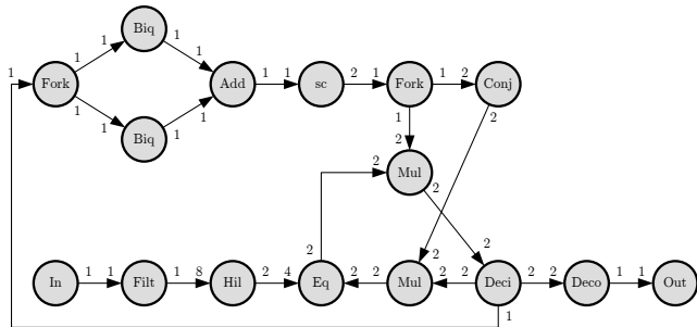
Figure 5: Modem application ([5])
