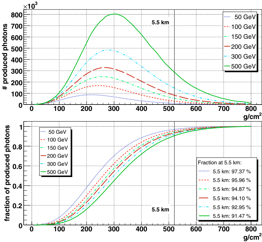
Fig. 1. In the upper plot , the number of produced photons (generated with CORSIKA Knapp & Heck 2004) is shown versus height (airmass in \text{g}/\text{cm}^2 ) for monoenergetic showers with energies between 50 GeV and 500 GeV in different colors. Below, the integral fraction of produced photons is plotted versus height for the same showers. In addition, the integral fraction of light at to 5.5 km, indicating the upper border of the Saharan Air Layer, is listed for each graph.
