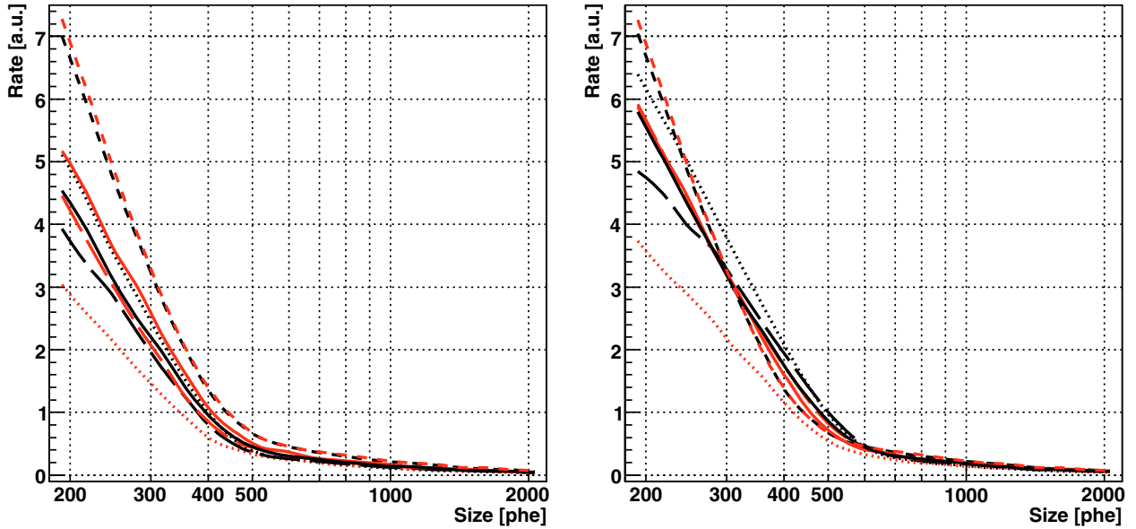
Fig. 3. SIZE distributions between 200 phe and 2000 phe (i.e. approximately from 100 GeV to 1 TeV) before ( left ) and after ( right ) correcting for the effect of SAL. Each line corresponds to one night and is scaled by the observation time. The color and style of each line is different to distinguish the nights from each other.
