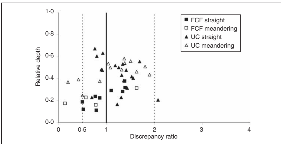
Fig. 13. Sediment discharges prediction with the Yang and Lim formula
