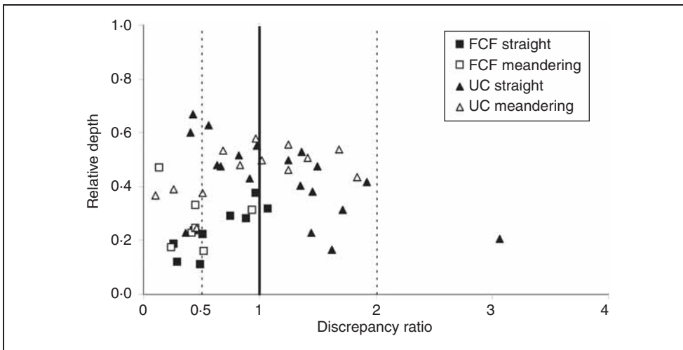
Fig. 11. Sediment discharges prediction with the Van Rijn formula (modified)
