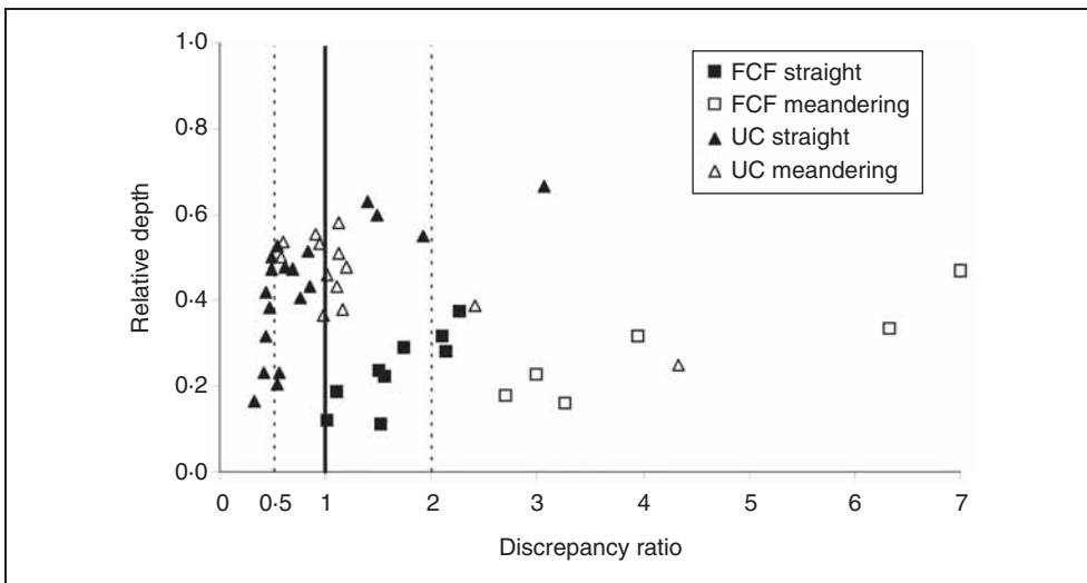
Fig. 7. Sediment discharges prediction with the Engelund and Hansen formula
