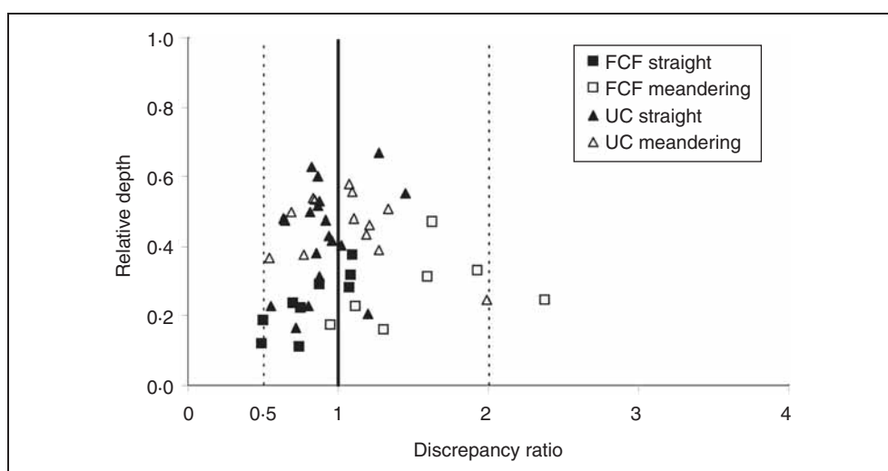
Fig. 10. Sediment discharges prediction with the Karim and Kennedy formula (with calibrated coefficient)
