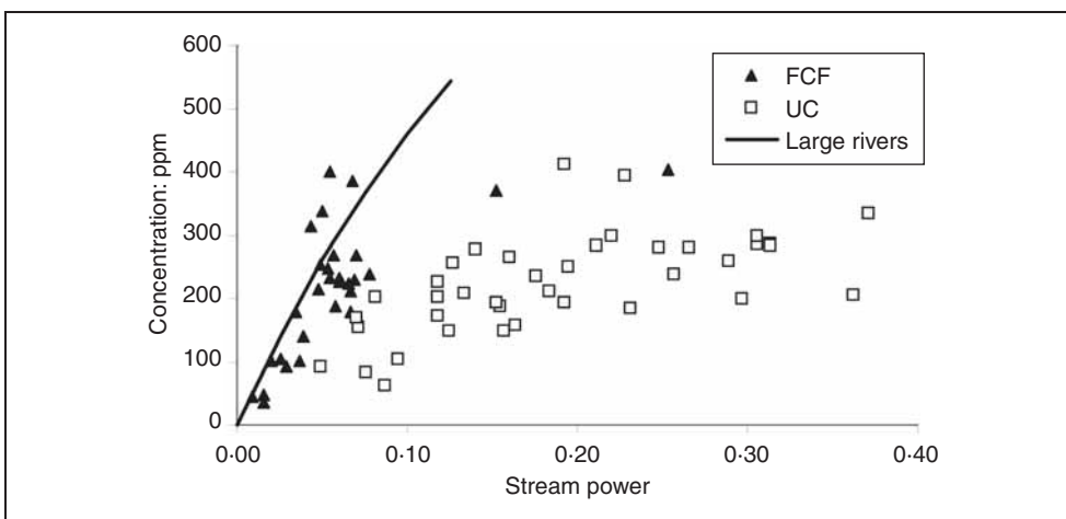
Fig. 12. Sediment discharges prediction with the Molinas and Wu formula
