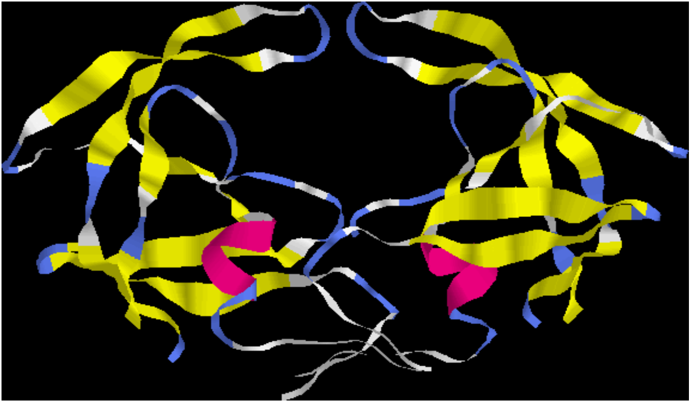
FIG. 1. Structure of HIV-1 PR [5].
