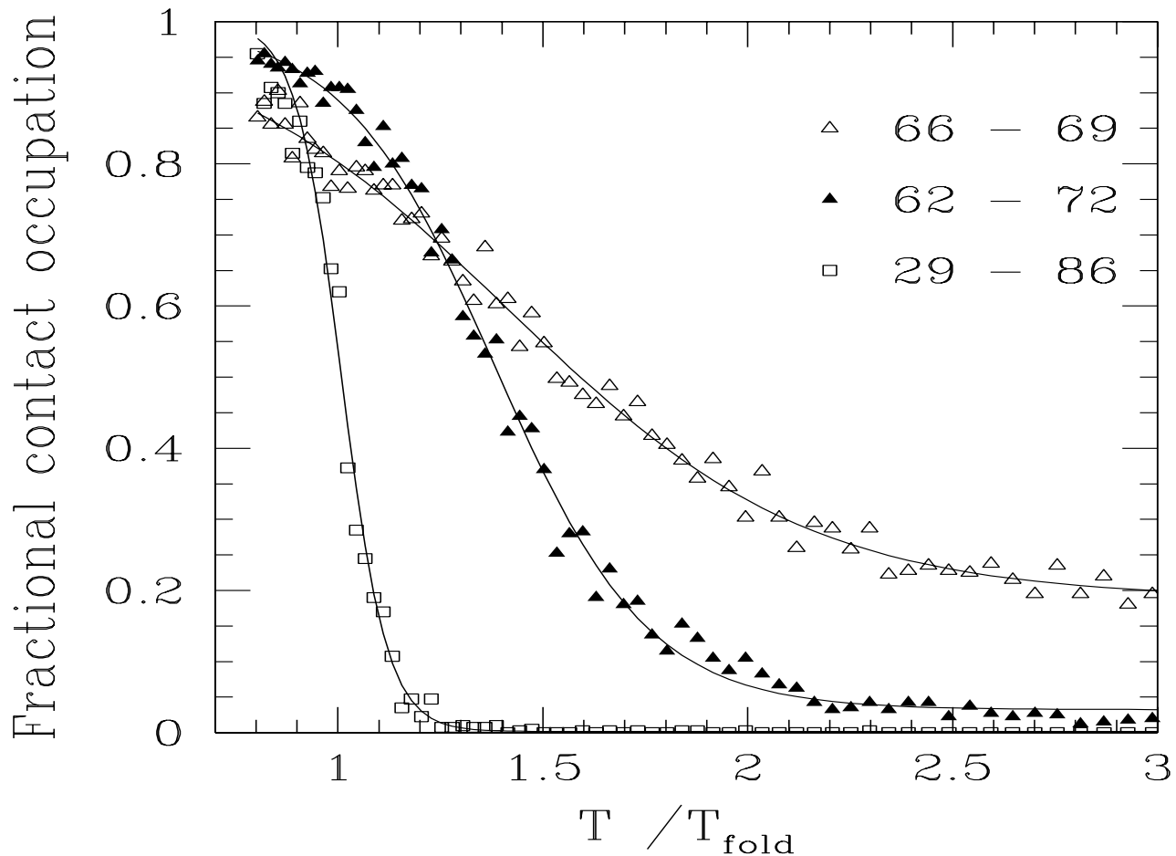
FIG. 2. Fractional occupation for three different native contacts. In all cases the fractional occupation approaches 1 as T \rightarrow 0 and vanishes for very large T . However, the rapidity of formation (slope at the inflexion point) is very different. The contact binding residues 66 and 69, located at the turn of \beta sheet 1, forms very gradually. The highest rapidity of formation of contacts in \beta_1 is observed for the pair 62, 72 (solid triangles). At the folding temperature, one of the highest formation rapidities is found in correspondence of the contact bonding residues 29 and 86 (open squares). The continuous curve is obtained from a smooth interpolation of the points.
