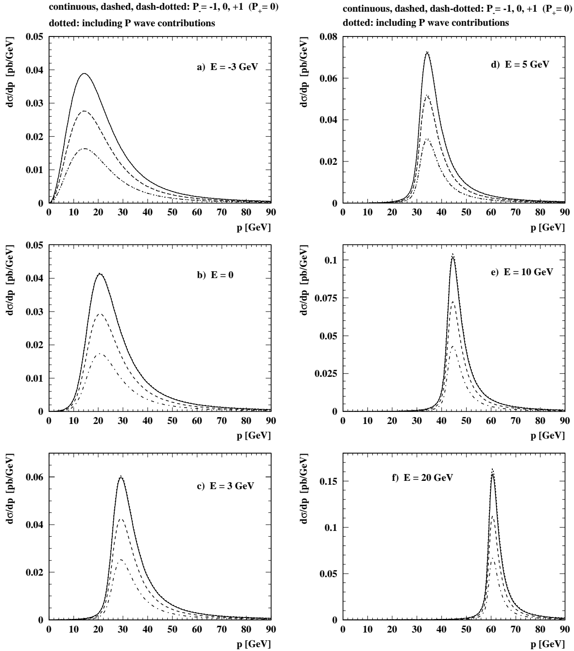
Figure 3: Differential cross section d\sigma(e^+e^- \rightarrow t\bar{t})/dp as defined in Eq. (1) as a function of p for six different energies, E = -3, 0, 3, 5, 10, 20 GeV, as indicated in the plots a)... f). The continuous, dashed and dash-dotted lines show the pure S wave result for the three different choices of the e^- polarization P_- = -1, 0 and 1 , respectively. ( P_+ = 0 .) The dotted lines show the full result including the P wave contributions.
