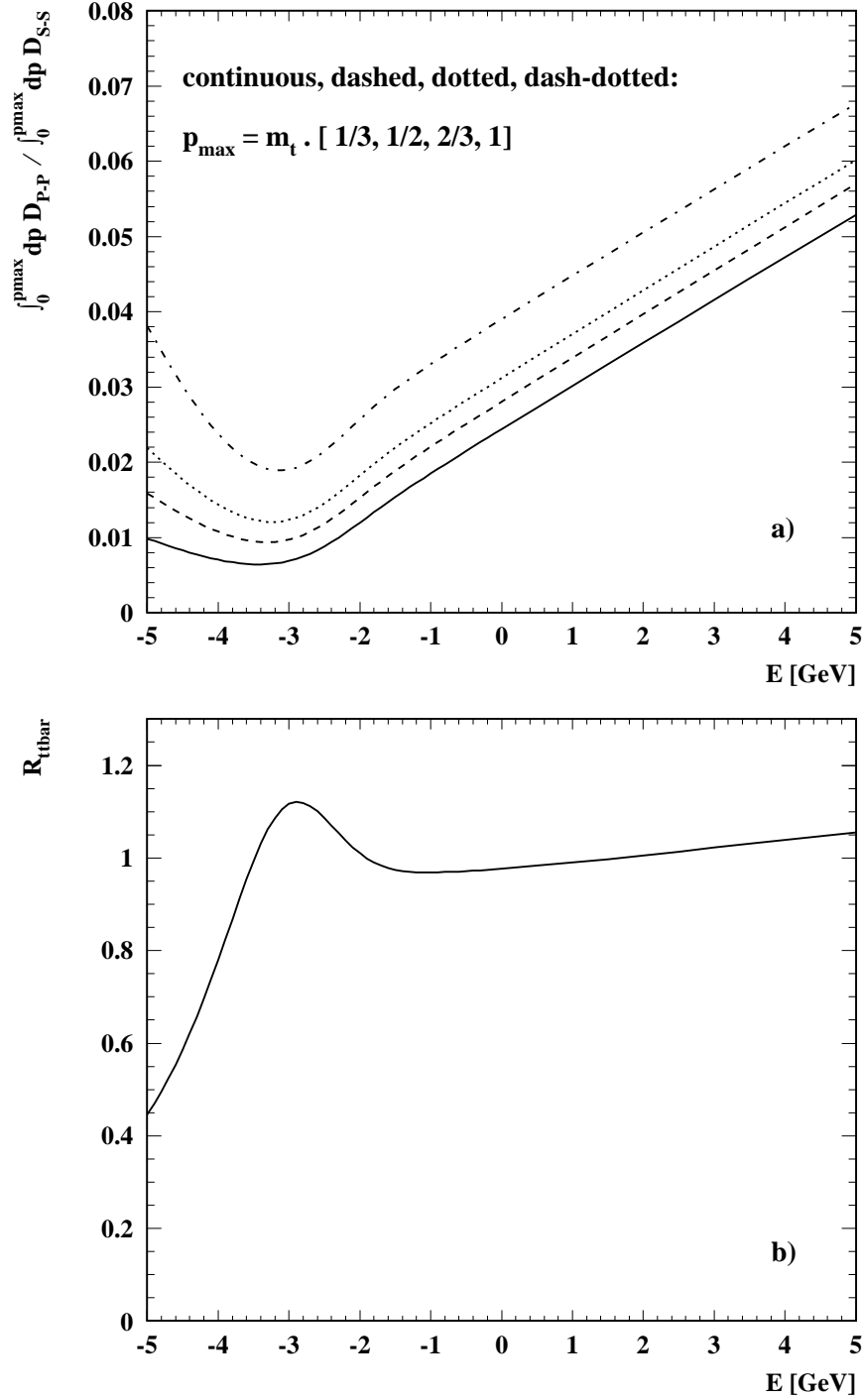
Figure 2: a) Ratio of the integrated distributions: \int_0^{p_{\max}} dp \mathcal{D}_{P-P}(p, E) / \int_0^{p_{\max}} dp \mathcal{D}_{S-S}(p, E) as a function of the energy E = \sqrt{s} - 2m_t for four different values of the cutoff: continuous, dashed, dotted, and dash-dotted lines correspond to p_{\max} = m_t \cdot [1/3, 1/2, 2/3, 1] , respectively. b) The normalized total cross section R_{t\bar{t}} as defined in Eq. (9) as a function of E .
