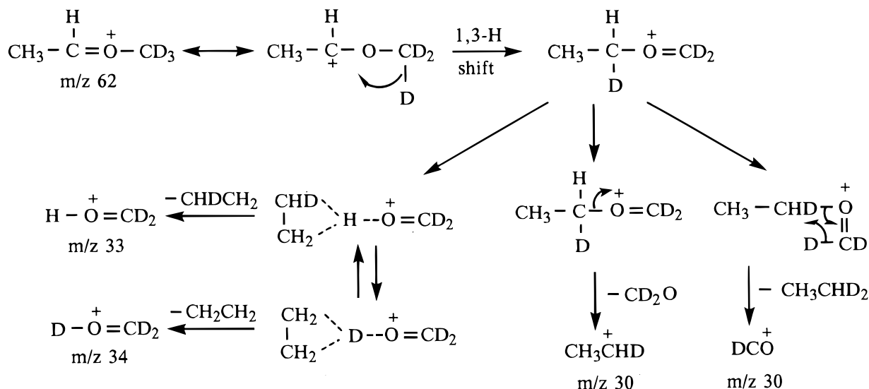
Scheme 2. Mechanisms proposed for the formation of the ions at m/z 30, 33 and 34 from the [\text{M} - \text{HCO}]^+ ion ( m/z 62) generated from the molecular ion of trideuteromethyl propanoate ( 1-d_3 ).
