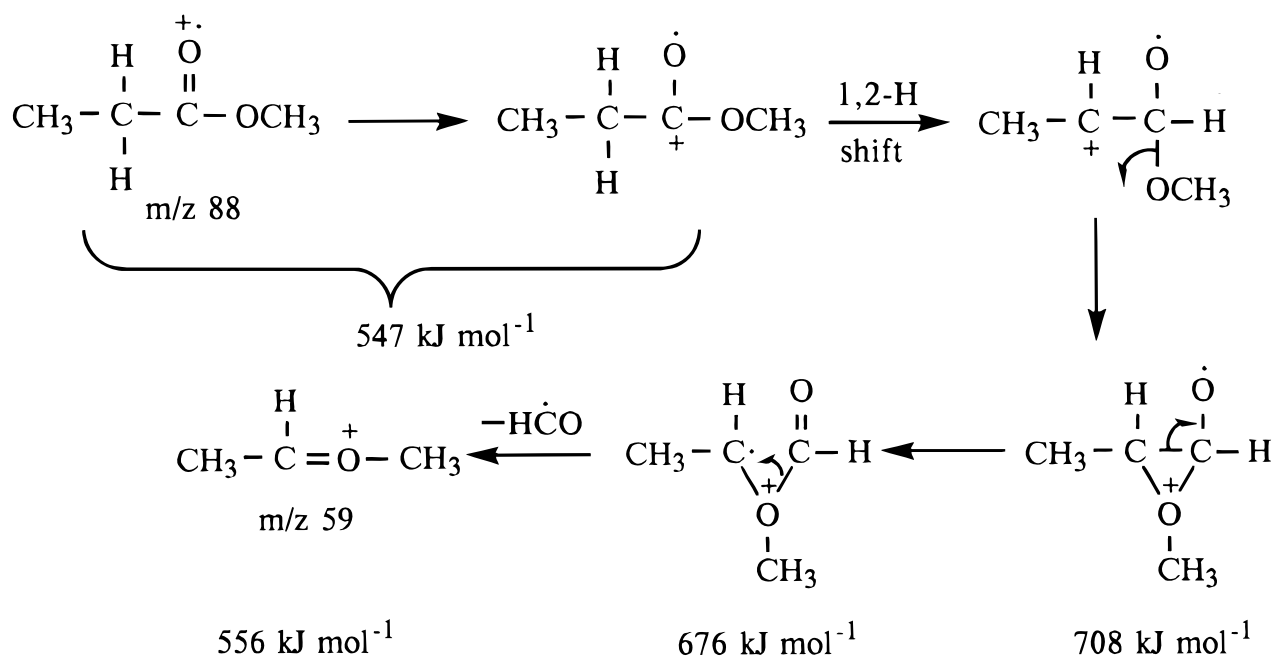
Scheme 1. Mechanism proposed for the loss of HCO from the molecular ion of methyl propanoate (1). The values given under the structures are the heats of formation calculated at the ROHF/6-31G* level of theory 16 with reference to the heat of formation of 1 + (547 kJ mol -1 ). 14 For the top-right structure no stable energy minimum has been obtained. The value of 556 kJ mol -1 for the bottom-left structure was taken from Ref. 15.
