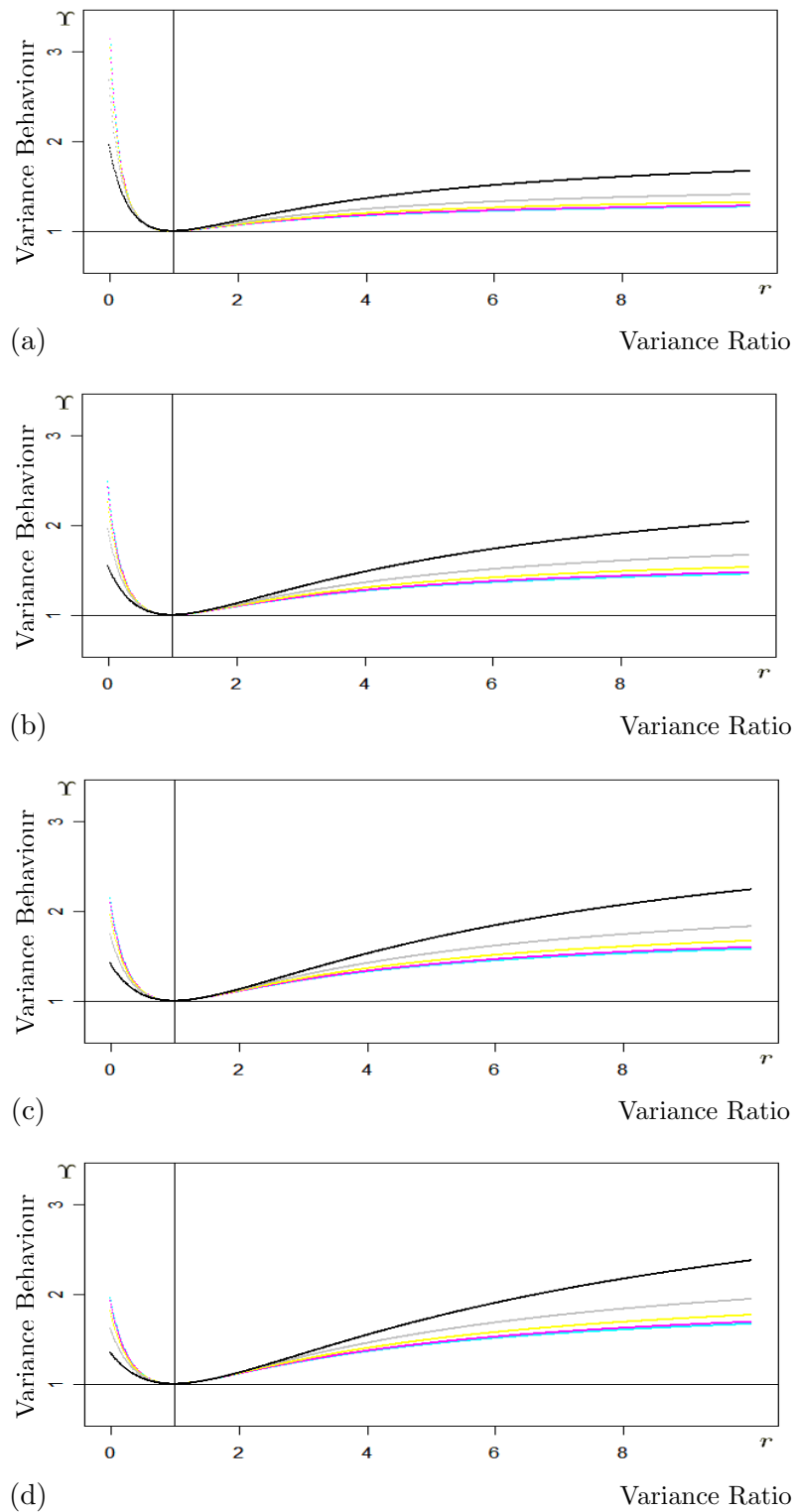
These Figures show the variance behaviour of the ratio of the real overall variance to the optimal value as r increases and under the assumption of 2 studies each of which with the same total number of patients N . The 5 lines represent different values of \beta ( - = 0.9, 0.1, - = 0.8, 0.2, - = 0.7, 0.3, - = 0.6, 0.4, - = 0.5 ) while \alpha is set equal to 0.1 (a), 0.2 (b), 0.3 (c) and 0.5(d).
