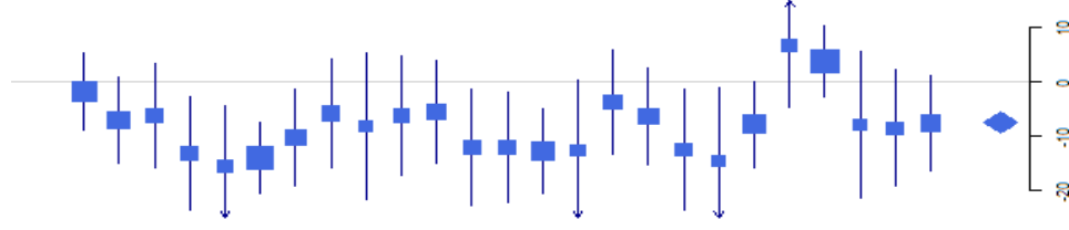
Figure 3.8: Effects of Treatment on FEV_1 for single-dose studies. Single doses of cardioselective \beta -blockers (divided in two groups; with or without intrinsic sympathomimetic activity) vs Placebo. Forest Plot: Mean Difference Estimates with 95% Intervals for the data of the 25 trials - The area of squares is proportional to the study precision. Fixed-Effects (test for heterogeneity, P = 0.09 ) meta-analysis on 25 studies; Compared with placebo, single doses of cardioselective \beta -blockers as a group were associated with a 7.43% (CI, 5.57% ,9.29%) ( P < 0.0001 ) reduction in FEV_1 .
