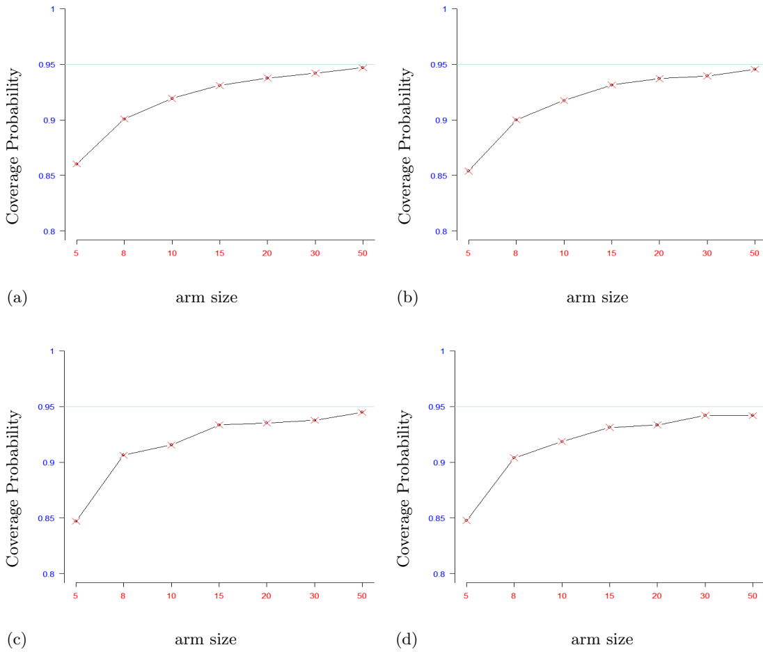
The figures show Estimated Coverage Probabilities of the Confidence Intervals based on 10000 simulation replicates. Different values of k –the number of trials – and n –the number of patients per arm, with n = n_C = n_T – are considered: (a) k = 10 , (b) k = 15 , (c) k = 25 , (d) k = 35 .
