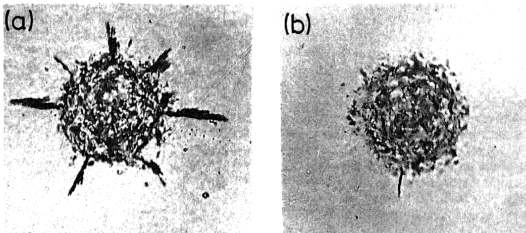
Figure 2 Radial cracks around a spherical indentation, (a) uncoated surface and (b) coated surface, (X 238).
