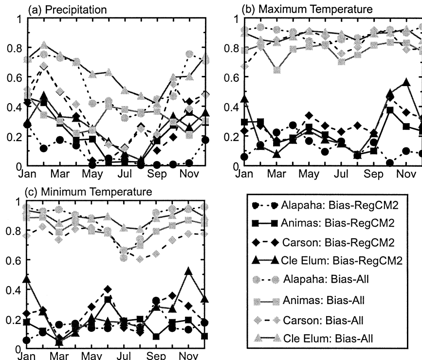
FIG. 10. The R-square values by month for each basin calculated using 1) bias-corrected RegCM2 and best three-station values and 2) bias-corrected all stations and best three-station values for (a) precipitation, (b) max temperature, and (c) min temperature.
