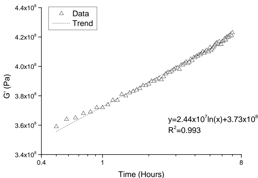
Figure 9. Change in shear storage modulus ( G' ) during isothermal holding at -20\text{ }^{\circ}\text{C} .
