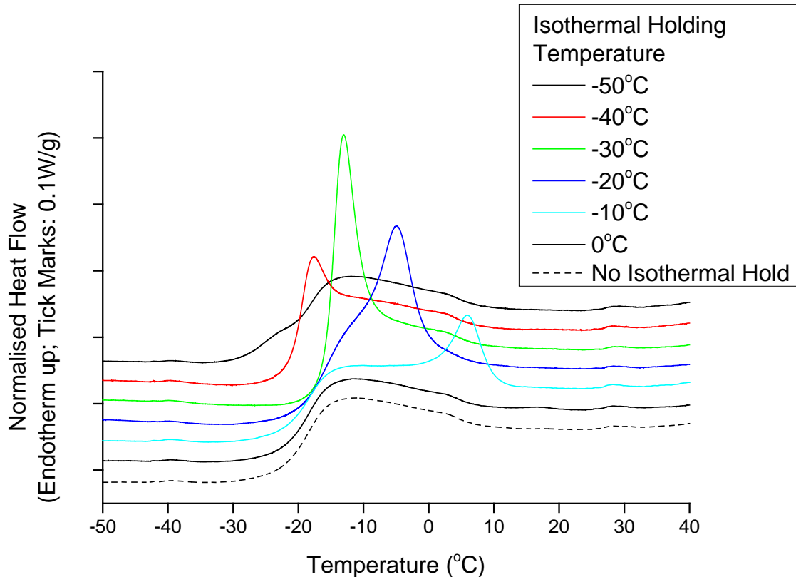
Figure 2. DSC results of the HNBR after isothermally holding for 24 hours at different temperatures. Curves are shifted vertically for clarity.
