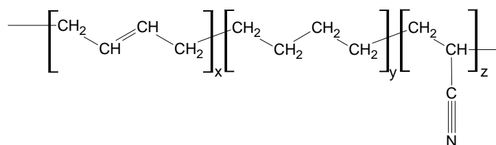
Figure 1. Simplified model of the structure of HNBR [9]. The ratio x:y indicating degree of saturation (residual double bonds), and z:(x + y) indicating the acrylonitrile content. Structures such as cis- and trans-isomers, pendant ethyl groups and chain branching are likely to also be present in HNBRs, but these are not shown in this simplified model.
