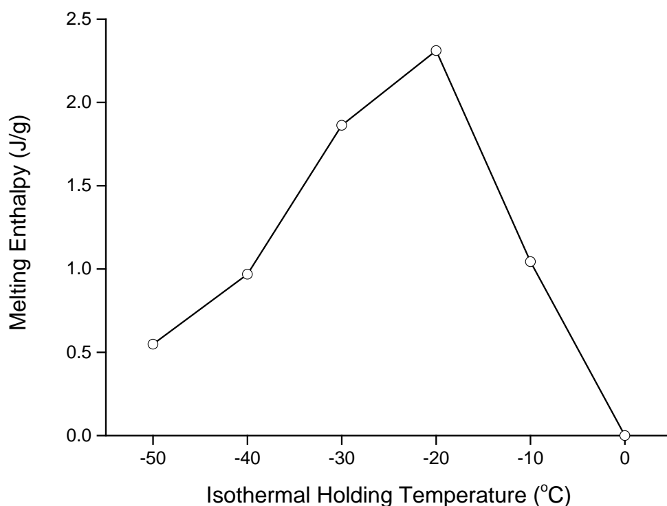
Figure 3. Melting enthalpies measured after isothermally holding for 24 hours at different temperatures.
