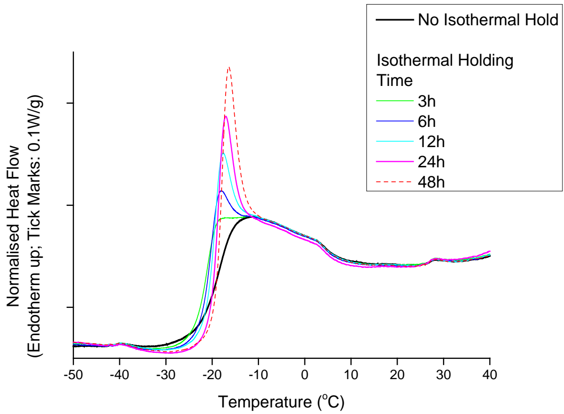
Figure 5. DSC results of the HNBR after isothermally holding at -40 °C for different holding times. Note the different scale of y-axis compared to Figure 4.
