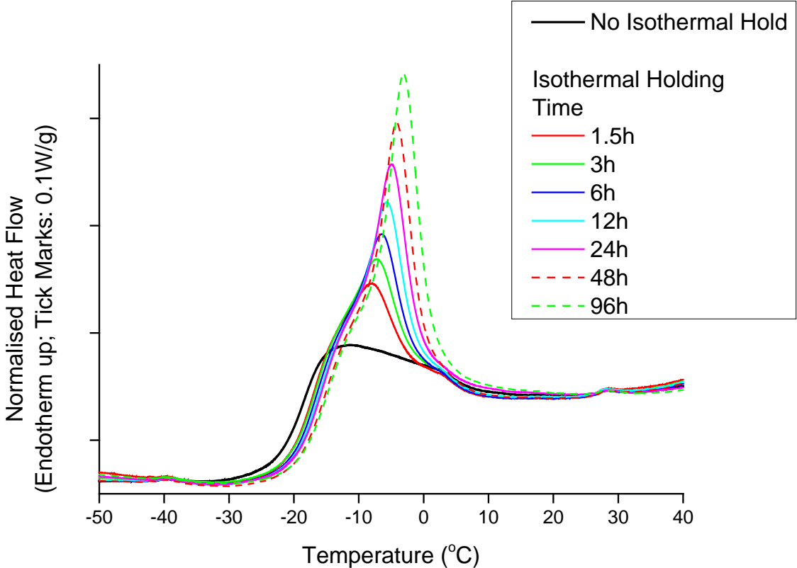
Figure 4. DSC results of the HNBR after isothermally holding at -20 °C for different holding times.
