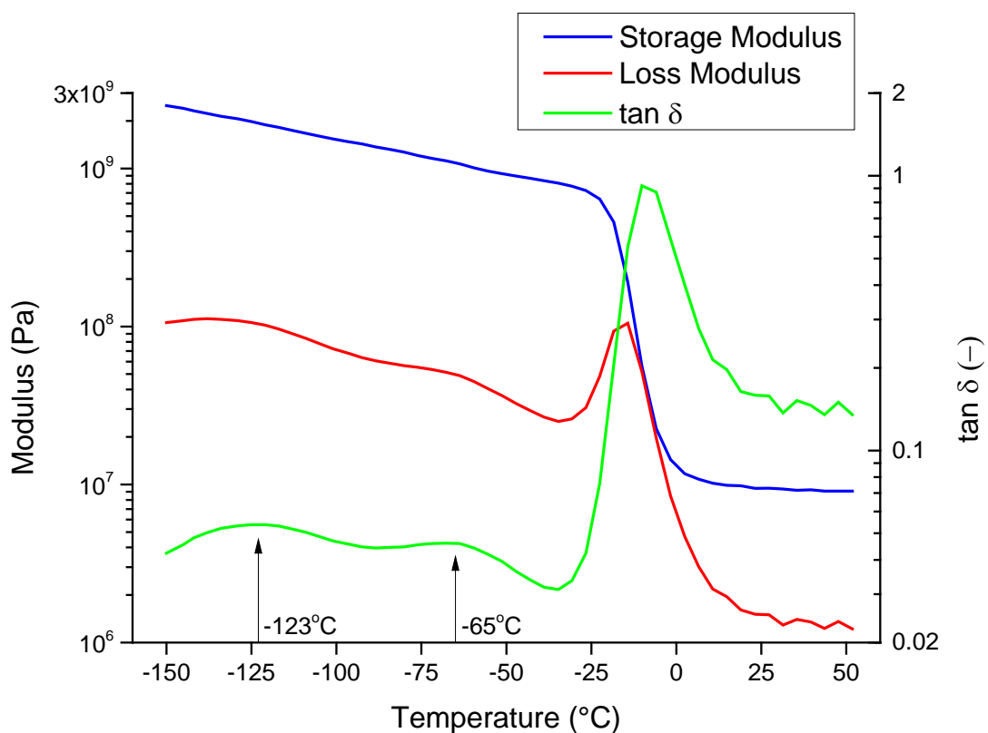
Figure 8. DMTA measurement of shear storage modulus ( G' ), shear loss modulus ( G'' ) and \tan \delta . The arrows indicate the peaks in \tan \delta referred to in the text.
