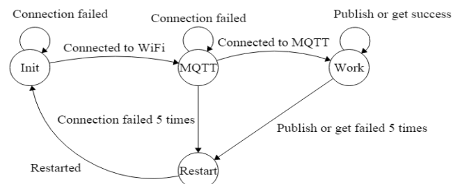
Fig. 4. ESP8266 finite state machine
