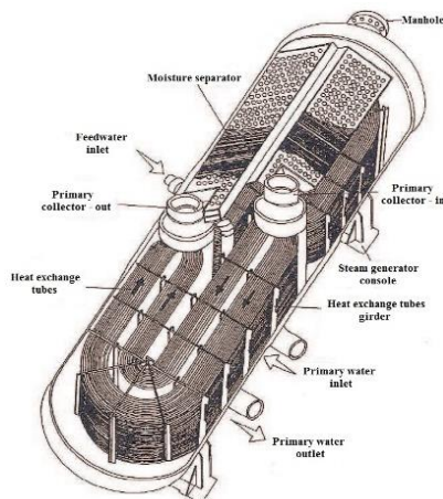
Fig. 1. Steam generator for NPPs with VVER-440 type reactor [23]
