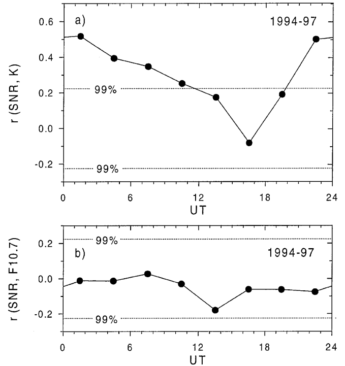
Fig. 3a, b. Diurnal variation of correlation coefficients between a SNR (83.0–87.5 km, Andenes) and geomagnetic K values and b between SNR and solar activity indices F10.7 using data for June and July 1994–1997. The dotted lines mark 99% significance levels
