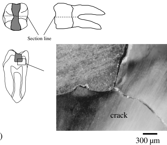
Fig. 1—Cracks evident along the internal line angles of two different restored molars. The crack orientation is perpendicular to the dentin tubule orientation in both molars
