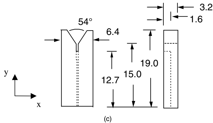
Fig. 3—Obtaining fatigue and fracture specimens from a bovine molar; all dimensions are in millimeters. Tubule orientation is defined with respect to the y -axis (i.e., the tubules for 0^\circ dentin are oriented parallel to the y -axis). (a) A sectioned bovine molar mounted in a polymer resin and an outline of a potential specimen from a single mesial-distal section; (b) DCB specimen; (c) WL-DCB specimen
