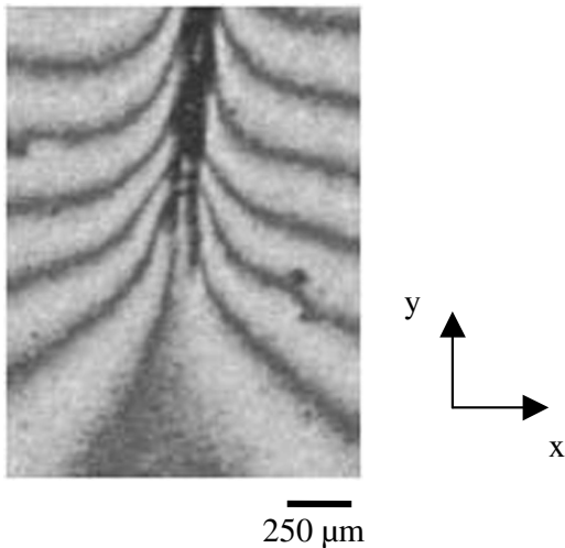
Fig. 9—A magnified view of the Moiré fringe patterns near the crack tip from Fig. 8(a). Note the prevalent non-linearity in the fringe pattern adjacent to the crack boundary
