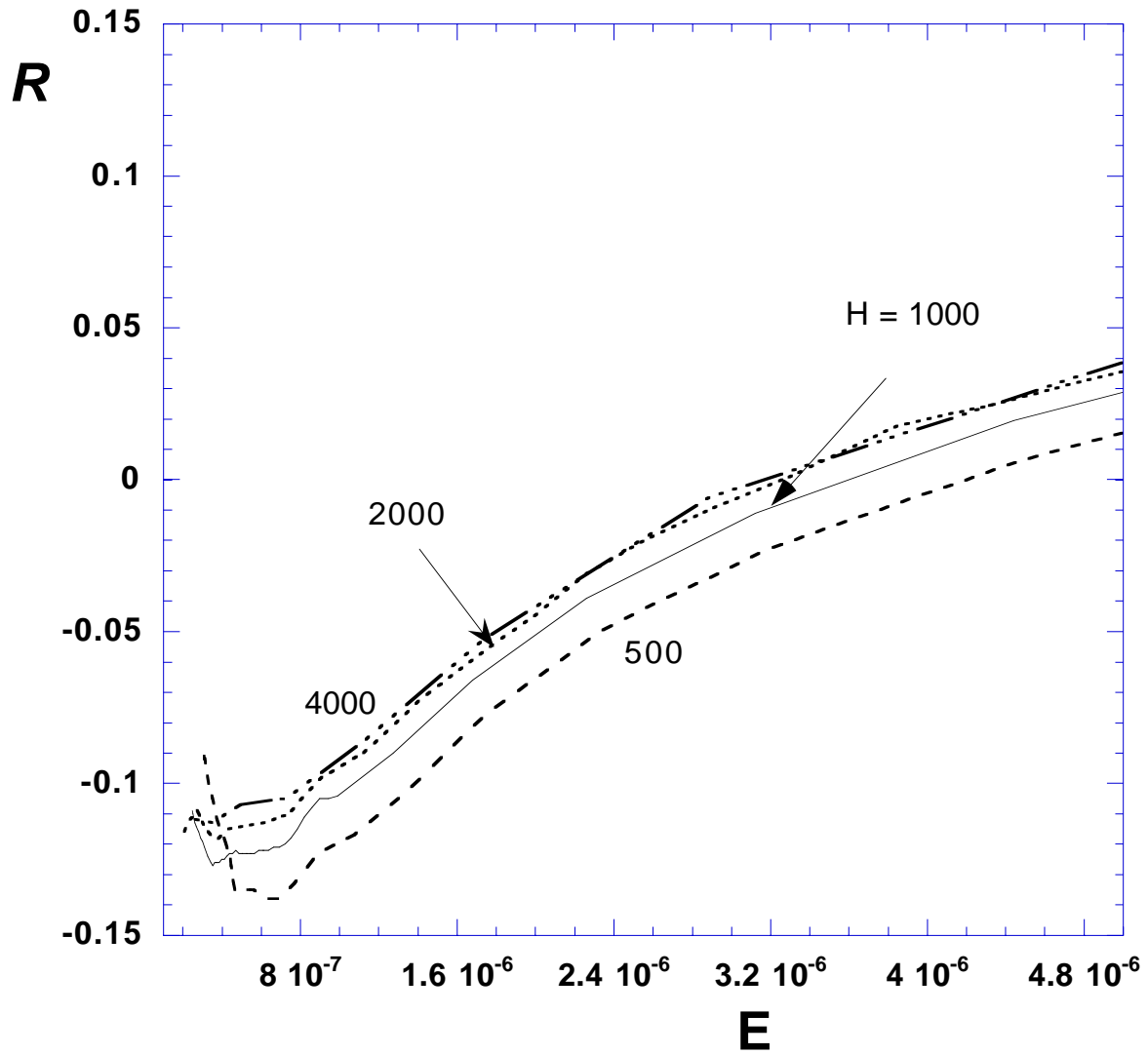
Figure 10: Bifurcation diagram showing the retroreflection index \mathcal{R} versus the Ekman number E for four different layer depths H .
