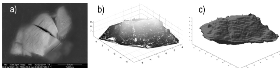
Figure 1. Deriving the 3D shape of a dust particle: a) SEM image of a micron-scale dust particle, b) topography retrieved using stereophotogrammetry, and c) volume-discretized shape, the lower half obtained by mirroring the shape with respect to the xy -plane.
