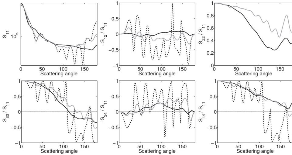
Figure 2. Comparison of scattering by single particles of different shapes. Scattering-matrix elements for the stereophotogrammetry-retrieved dust particle (solid black line) of size parameter x = 8.0 are shown together with those of an equal-volume Gaussian random sphere (solid gray line) and a spherical particle (dashed line).
