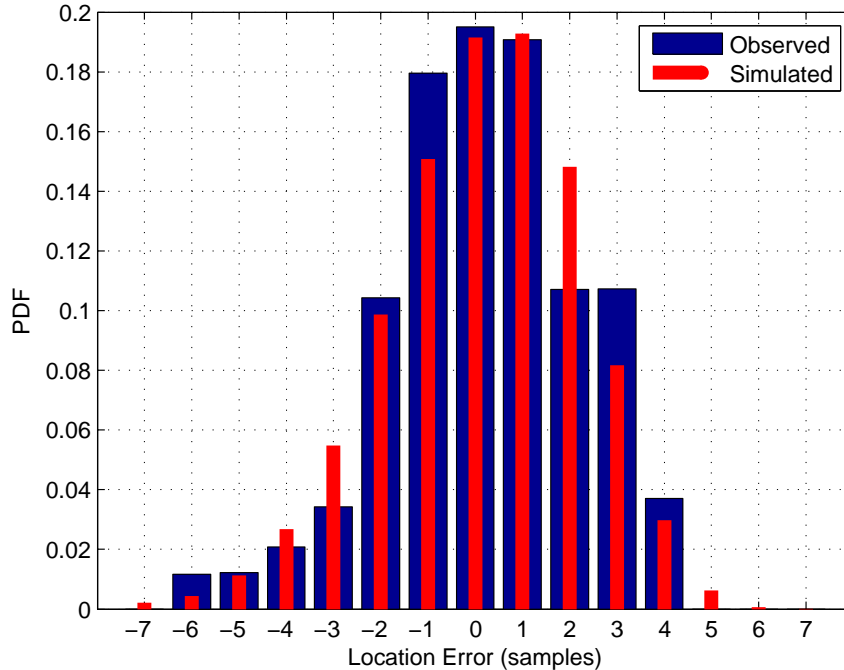
Figure 4.21: Histogram of observed burst location error in 9134 collected 802.11A bursts from four Cisco devices. Simulated error results for the four-parameter discrete Beta distribution are overlaid for comparison.
