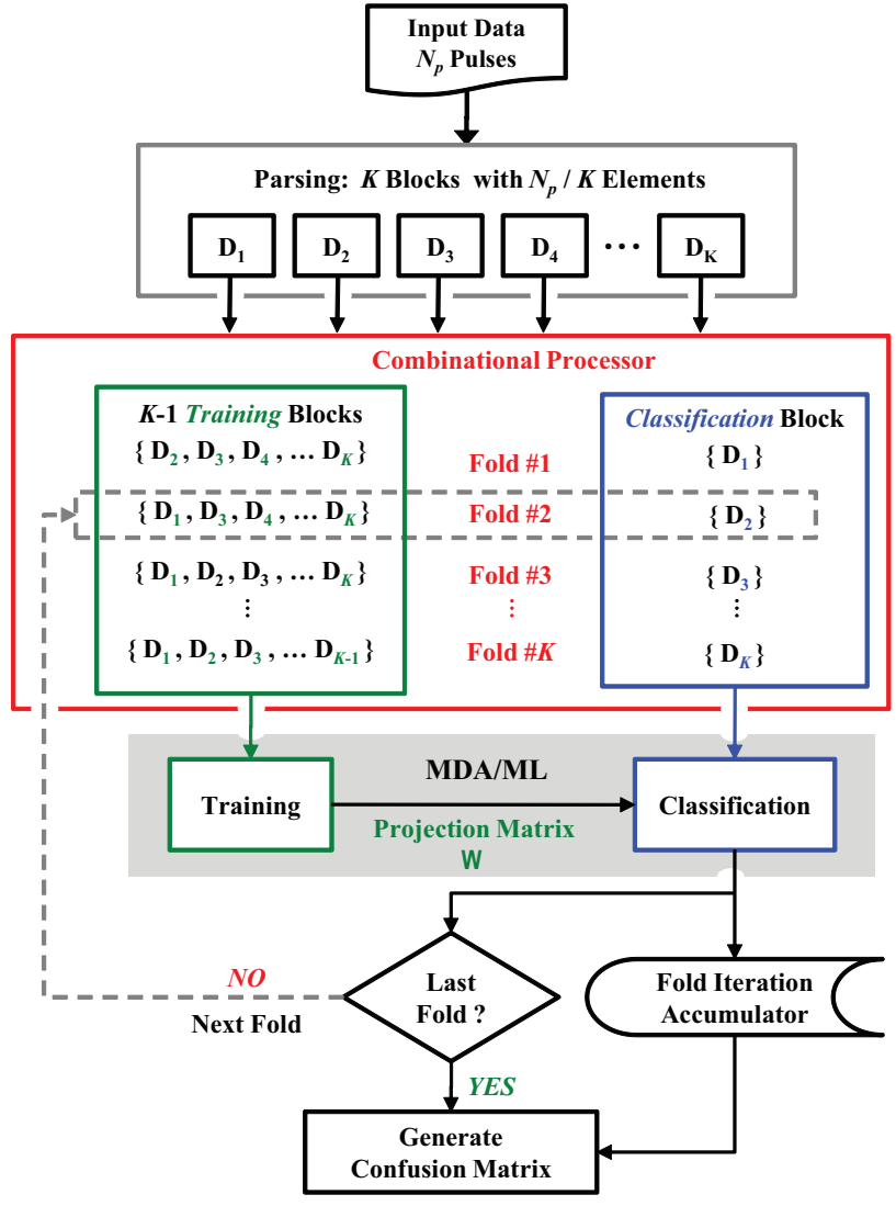
Figure 3.5: MDA/ML classification process with K-fold cross validation [71].
