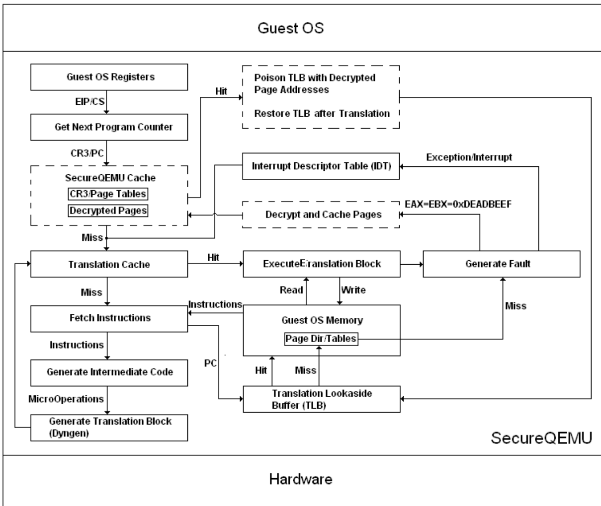
Figure 3.6: SecureQEMU Internals
